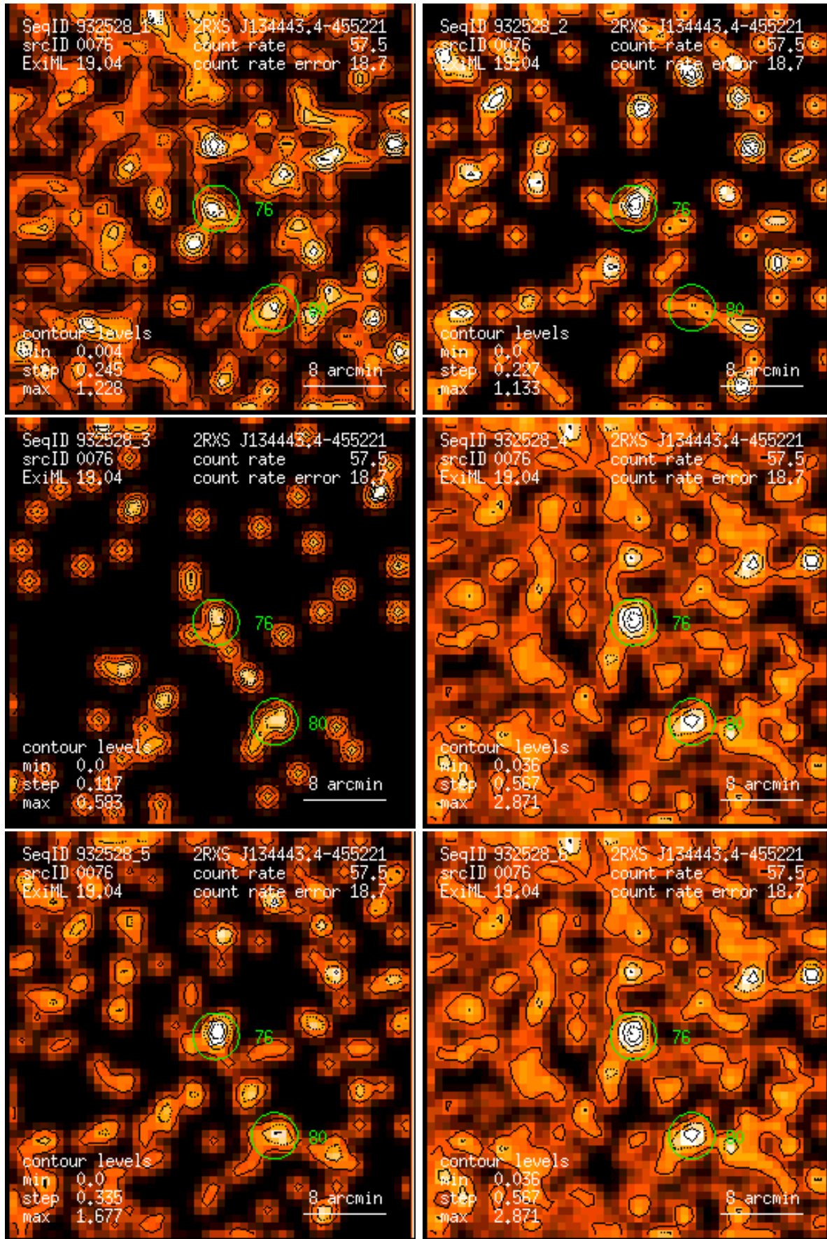
Figure 76: RASS 932528: detection 0076: band rate images, Gaussian filter: (1) PSPC channels 11 – 41, (2) 52 – 90, (3) 91 – 201, (4) 11 – 235, (5) 52 – 201, (6) 11 – 201. Broad band rates in counts/ks. Band rate contour levels in counts/ks/arcmin 2 .
