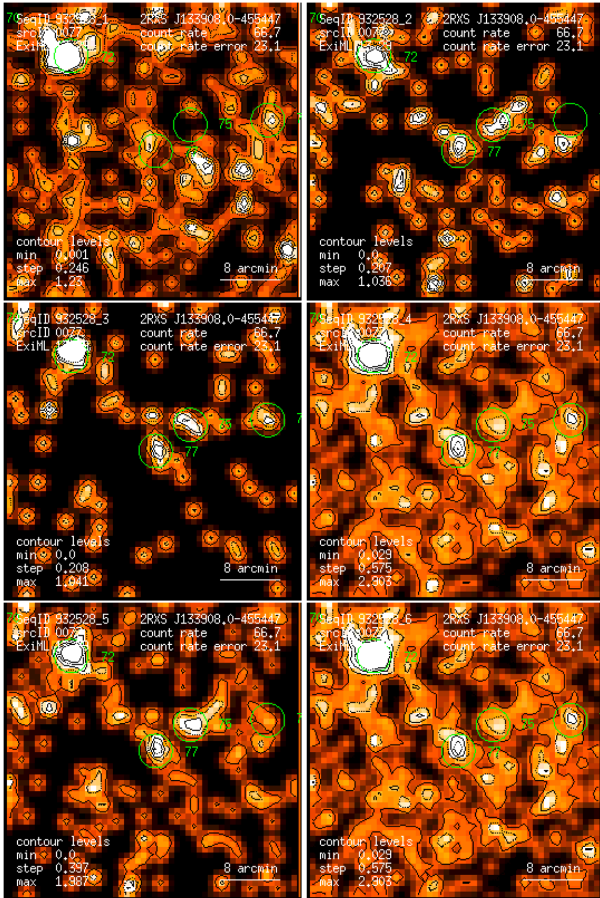
Figure 77: RASS 932528: detection 0077: band rate images, Gaussian filter: (1) PSPC channels 11 – 41, (2) 52 – 90, (3) 91 – 201, (4) 11 – 235, (5) 52 – 201, (6) 11 – 201. Broad band rates in counts/ks. Band rate contour levels in counts/ks/arcmin 2 .
