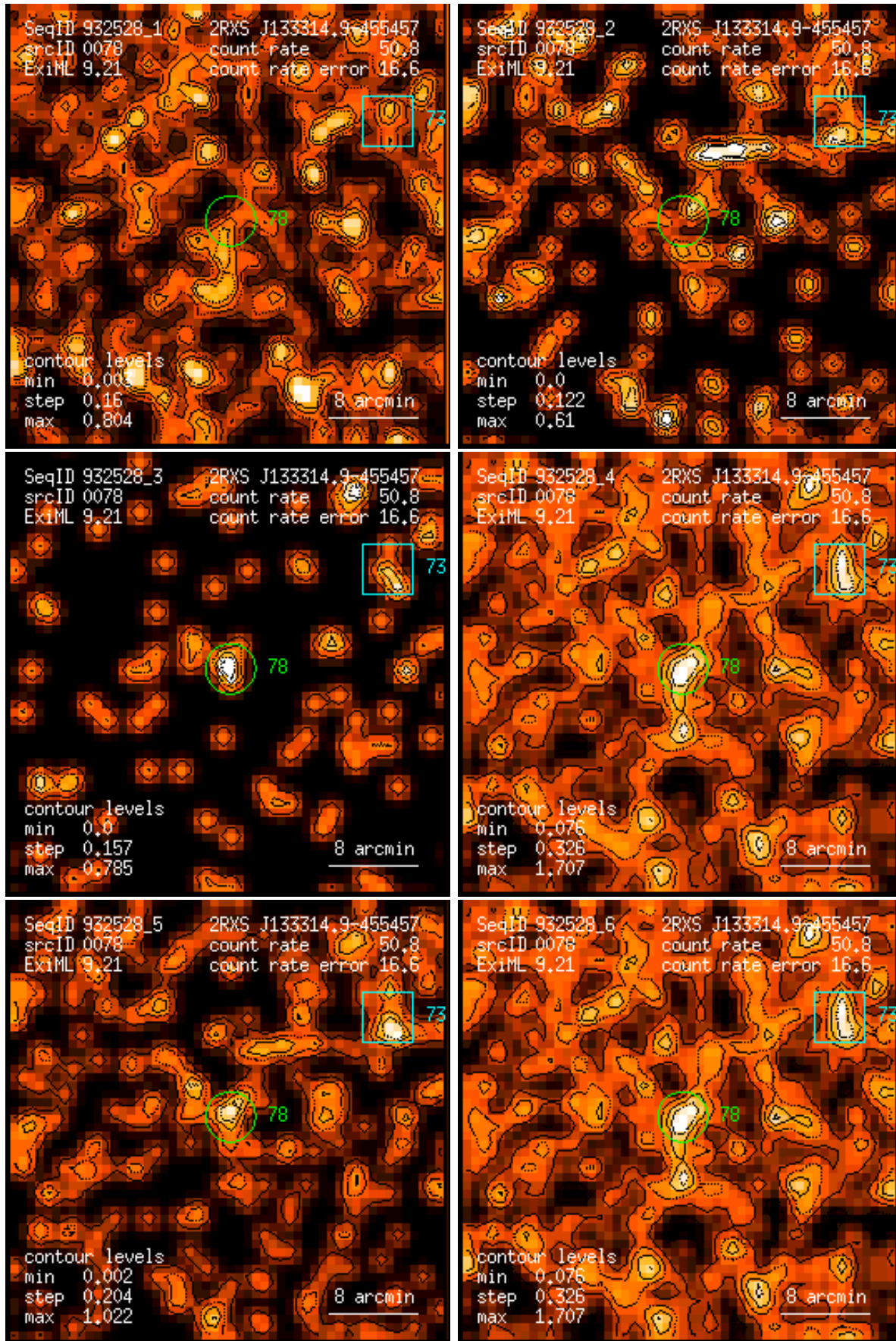
Figure 78: RASS 932528: detection 0078: band rate images, Gaussian filter: (1) PSPC channels 11 – 41, (2) 52 – 90, (3) 91 – 201, (4) 11 – 235, (5) 52 – 201, (6) 11 – 201. Broad band rates in counts/ks. Band rate contour levels in counts/ks/arcmin 2 .
