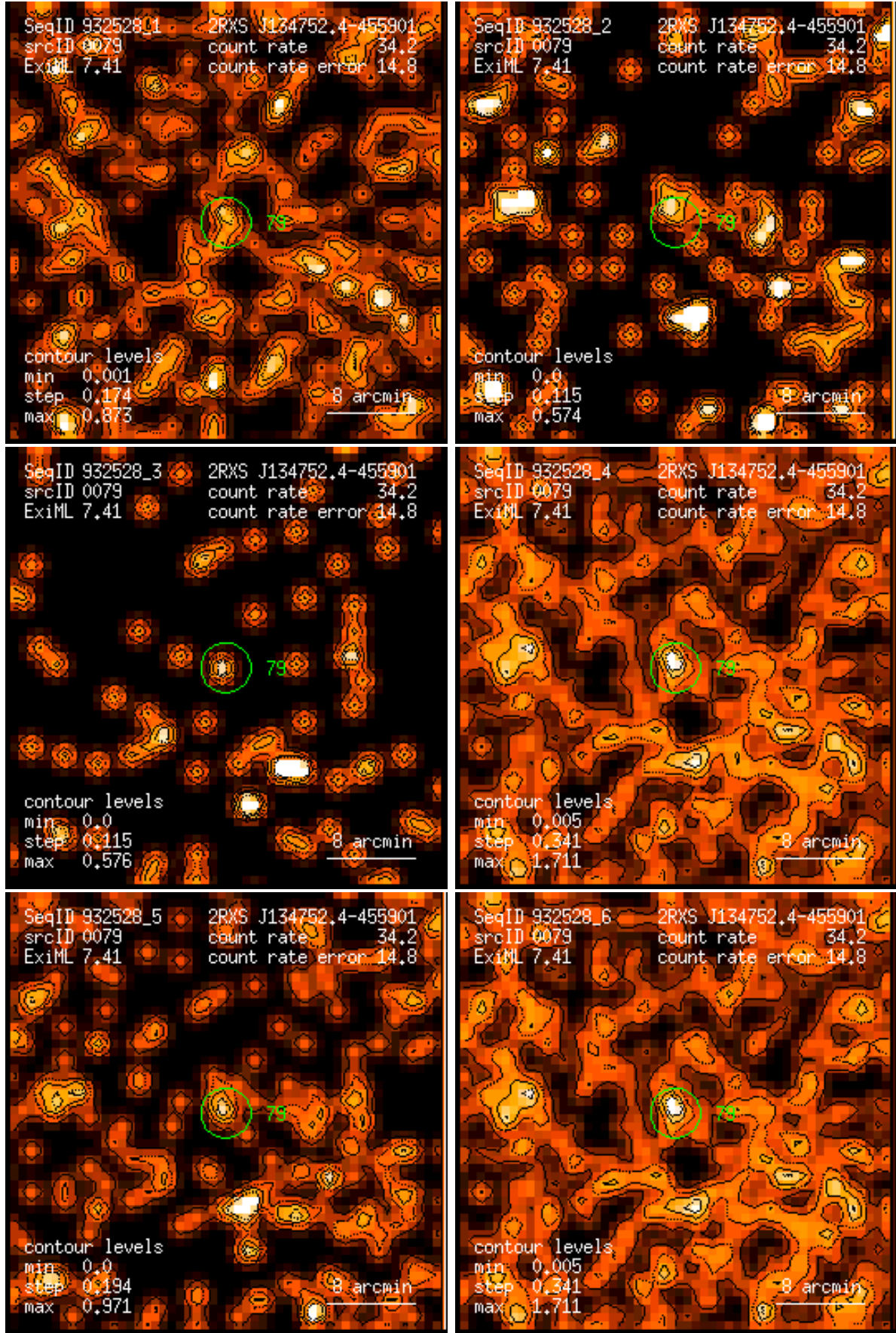
Figure 79: RASS 932528: detection 0079: band rate images, Gaussian filter: (1) PSPC channels 11 – 41, (2) 52 – 90, (3) 91 – 201, (4) 11 – 235, (5) 52 – 201, (6) 11 – 201. Broad band rates in counts/ks. Band rate contour levels in counts/ks/arcmin 2 .
