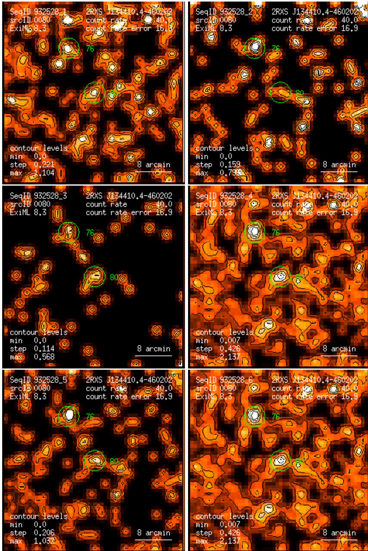
Figure 80: RASS 932528: detection 0080: band rate images, Gaussian filter: (1) PSPC channels 11 – 41, (2) 52 – 90, (3) 91 – 201, (4) 11 – 235, (5) 52 – 201, (6) 11 – 201. Broad band rates in counts/ks. Band rate contour levels in counts/ks/arcmin 2 .
