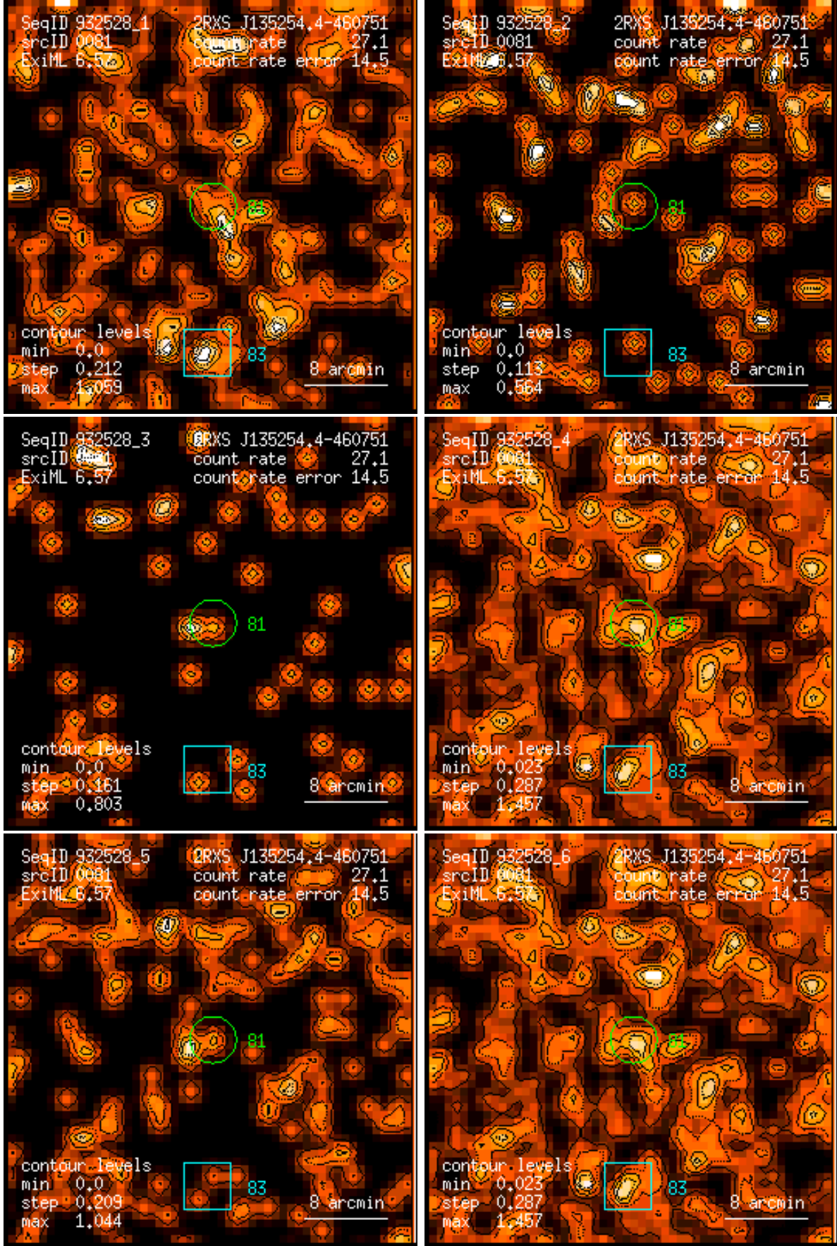
Figure 81: RASS 932528: detection 0081: band rate images, Gaussian filter: (1) PSPC channels 11 – 41, (2) 52 – 90, (3) 91 – 201, (4) 11 – 235, (5) 52 – 201, (6) 11 – 201. Broad band rates in counts/ks. Band rate contour levels in counts/ks/arcmin 2 .
