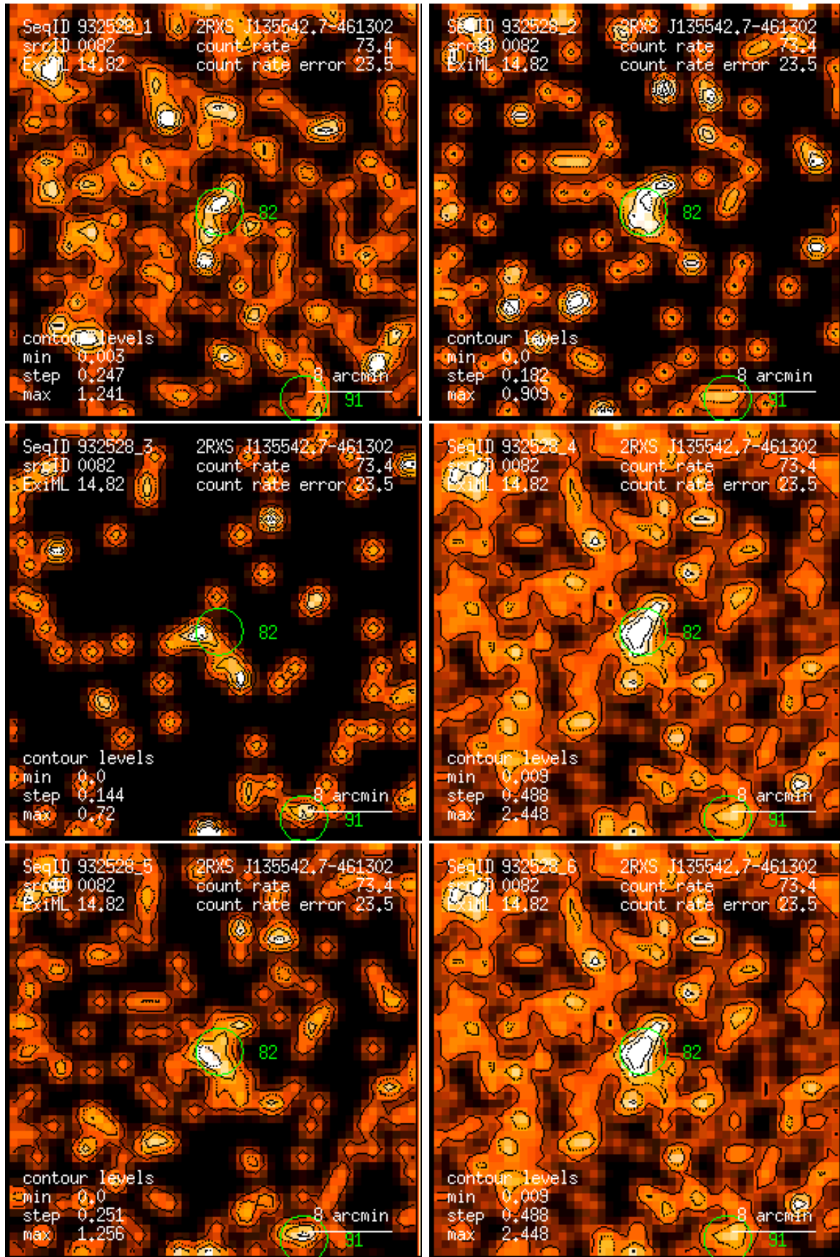
Figure 82: RASS 932528: detection 0082: band rate images, Gaussian filter: (1) PSPC channels 11 – 41, (2) 52 – 90, (3) 91 – 201, (4) 11 – 235, (5) 52 – 201, (6) 11 – 201. Broad band rates in counts/ks. Band rate contour levels in counts/ks/arcmin 2 .
