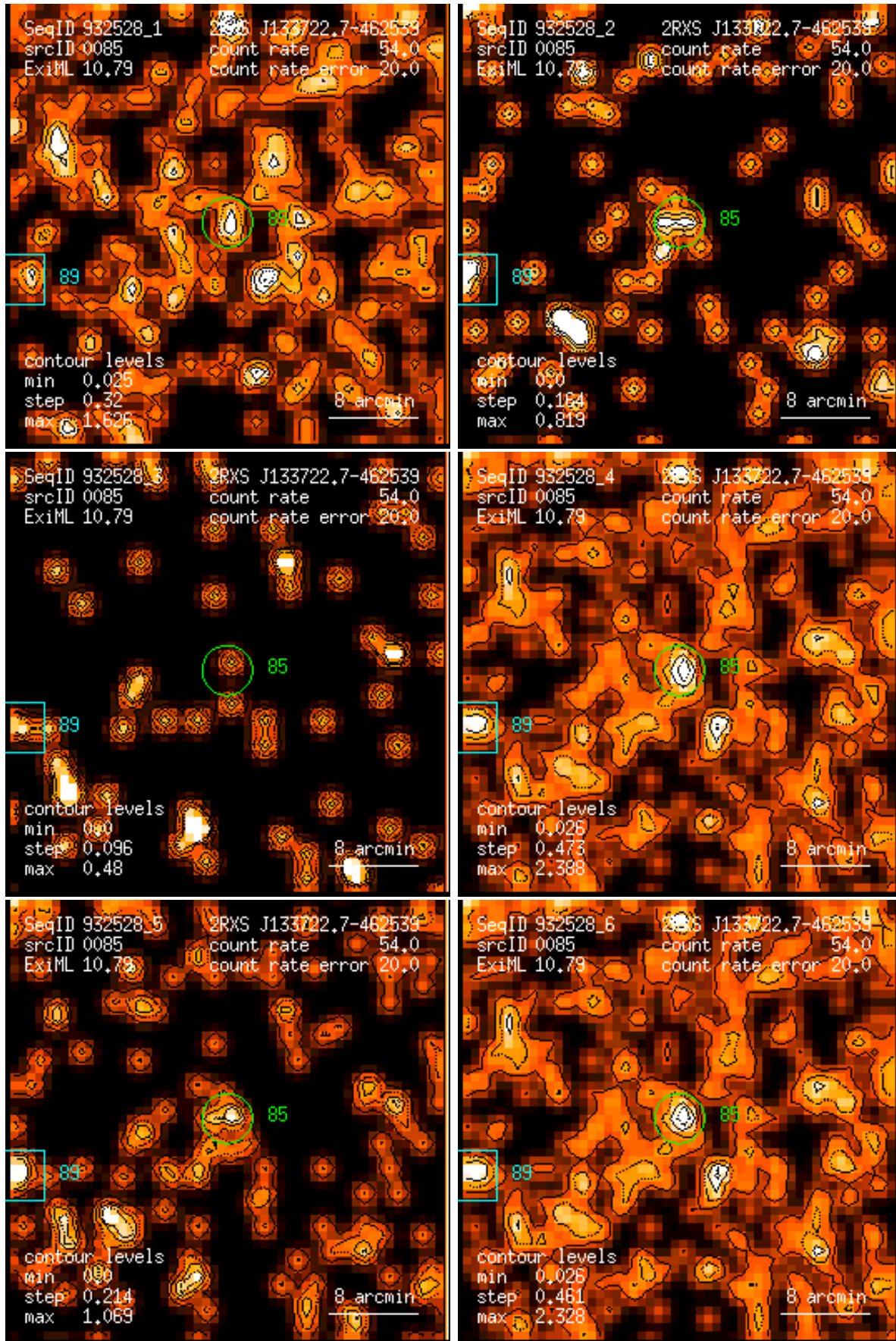
Figure 85: RASS 932528: detection 0085: band rate images, Gaussian filter: (1) PSPC channels 11 – 41, (2) 52 – 90, (3) 91 – 201, (4) 11 – 235, (5) 52 – 201, (6) 11 – 201. Broad band rates in counts/ks. Band rate contour levels in counts/ks/arcmin 2 .
