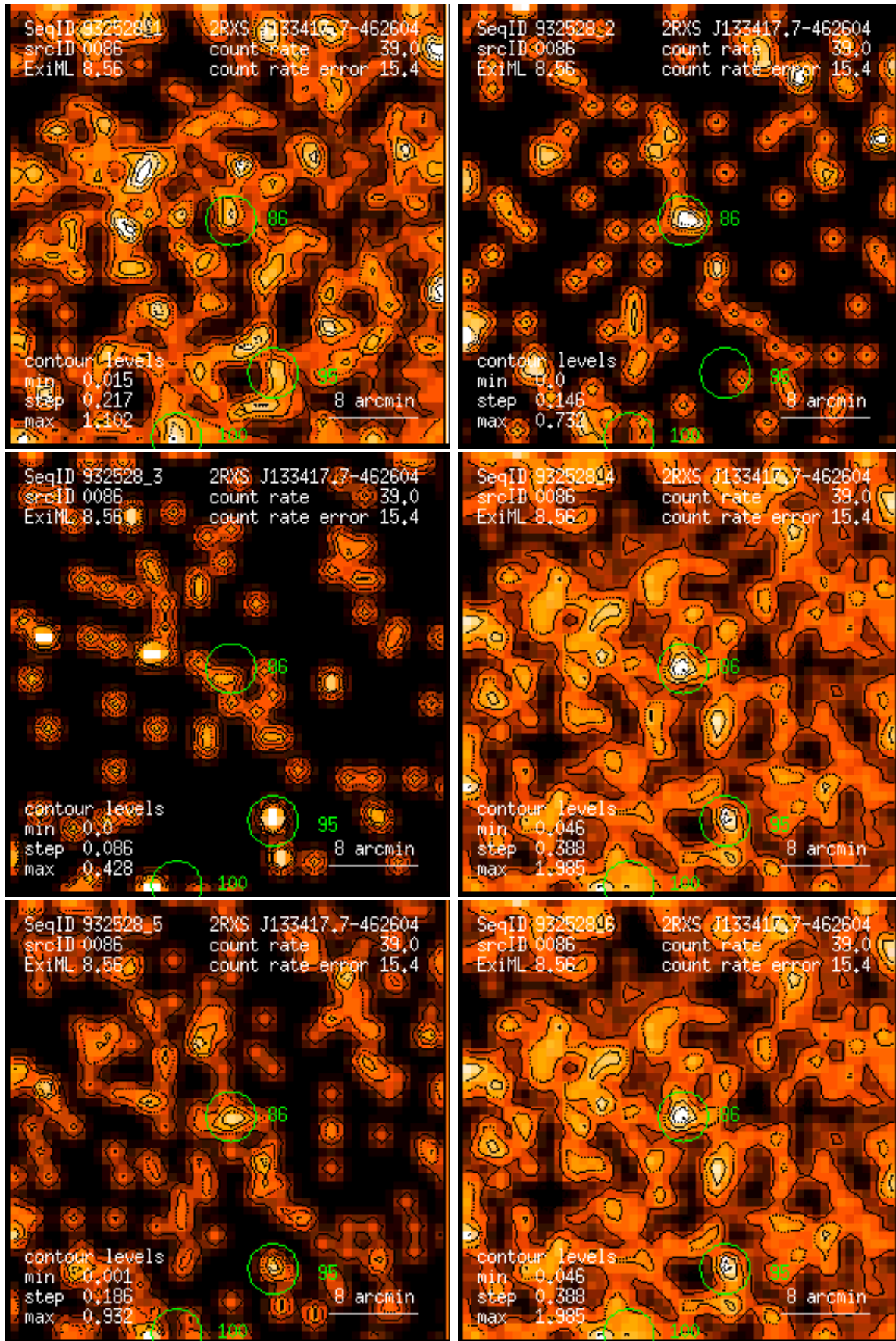
Figure 86: RASS 932528: detection 0086: band rate images, Gaussian filter: (1) PSPC channels 11 – 41, (2) 52 – 90, (3) 91 – 201, (4) 11 – 235, (5) 52 – 201, (6) 11 – 201. Broad band rates in counts/ks. Band rate contour levels in counts/ks/arcmin 2 .
