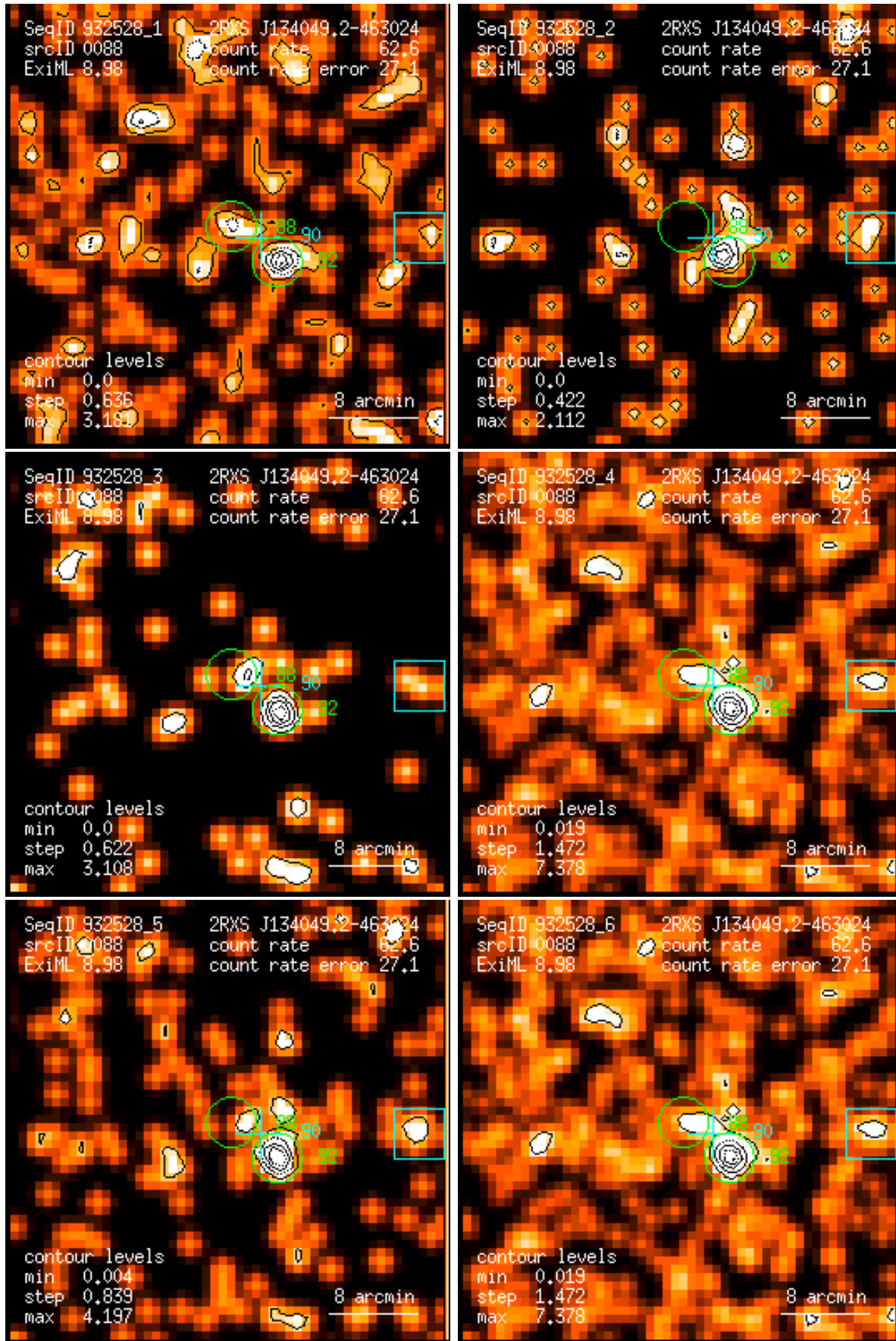
Figure 88: RASS 932528: detection 0088: band rate images, Gaussian filter: (1) PSPC channels 11 – 41, (2) 52 – 90, (3) 91 – 201, (4) 11 – 235, (5) 52 – 201, (6) 11 – 201. Broad band rates in counts/ks. Band rate contour levels in counts/ks/arcmin 2 .
