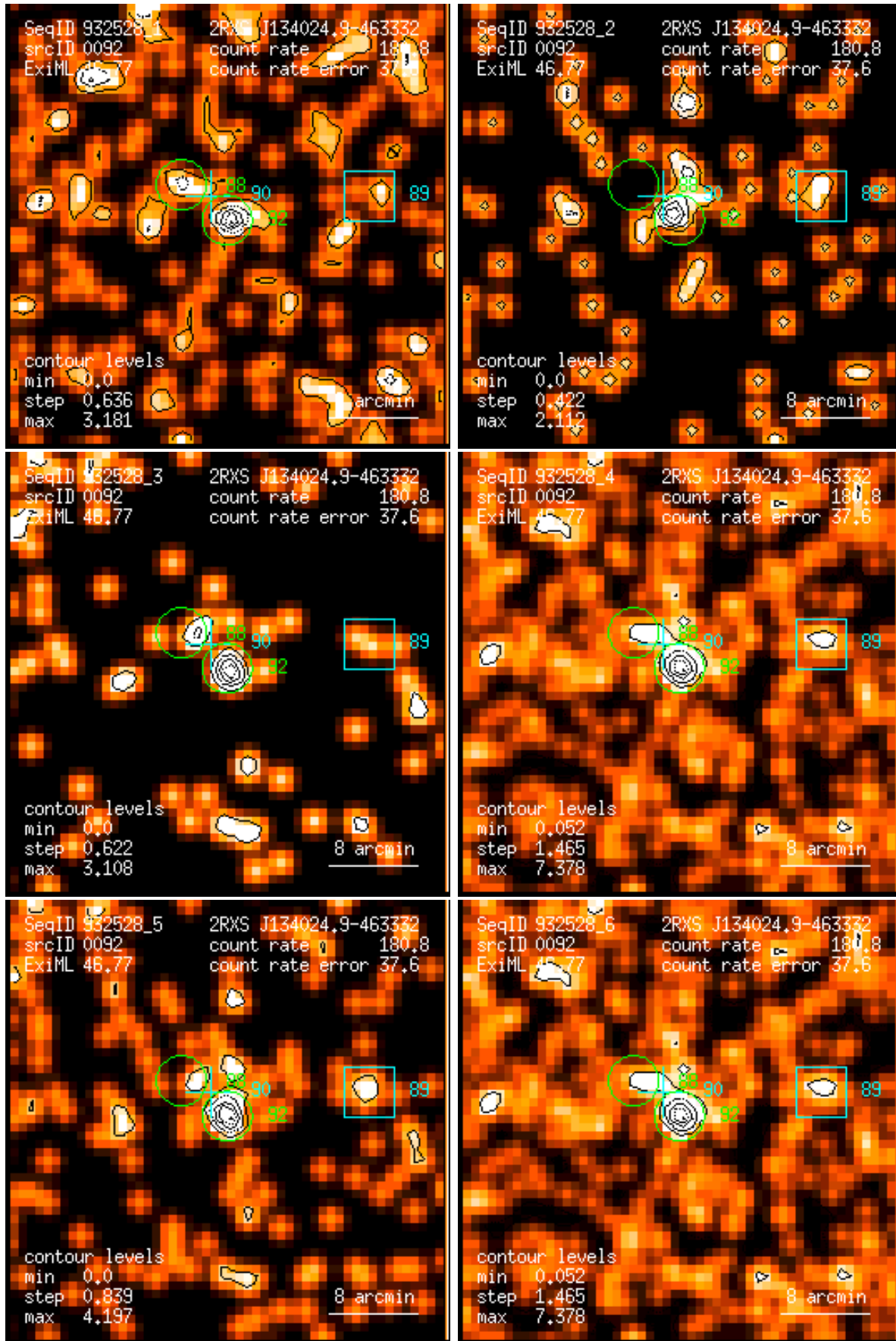
Figure 92: RASS 932528: detection 0092: band rate images, Gaussian filter: (1) PSPC channels 11 – 41, (2) 52 – 90, (3) 91 – 201, (4) 11 – 235, (5) 52 – 201, (6) 11 – 201. Broad band rates in counts/ks. Band rate contour levels in counts/ks/arcmin 2 .
