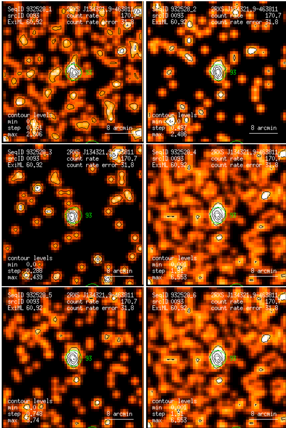
Figure 93: RASS 932528: detection 0093: band rate images, Gaussian filter: (1) PSPC channels 11 – 41, (2) 52 – 90, (3) 91 – 201, (4) 11 – 235, (5) 52 – 201, (6) 11 – 201. Broad band rates in counts/ks. Band rate contour levels in counts/ks/arcmin 2 .
