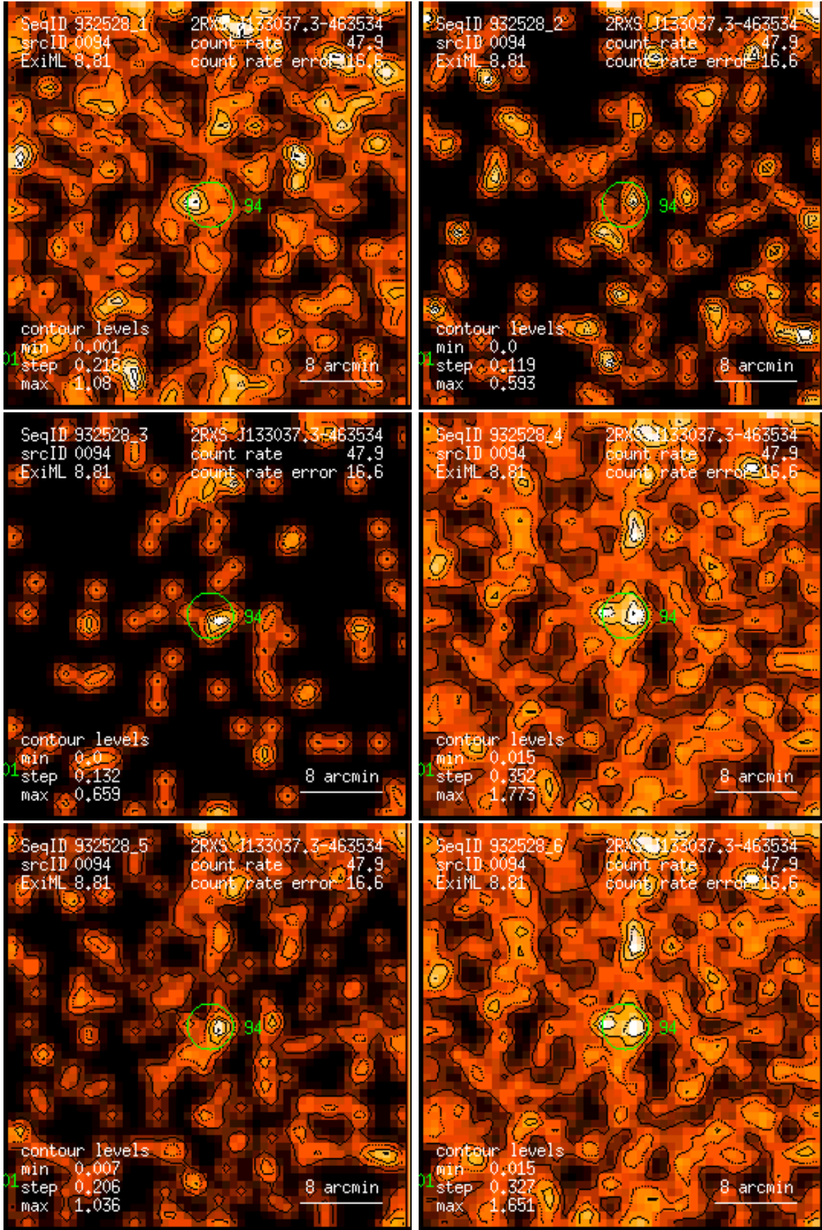
Figure 94: RASS 932528: detection 0094: band rate images, Gaussian filter: (1) PSPC channels 11 – 41, (2) 52 – 90, (3) 91 – 201, (4) 11 – 235, (5) 52 – 201, (6) 11 – 201. Broad band rates in counts/ks. Band rate contour levels in counts/ks/arcmin 2 .
