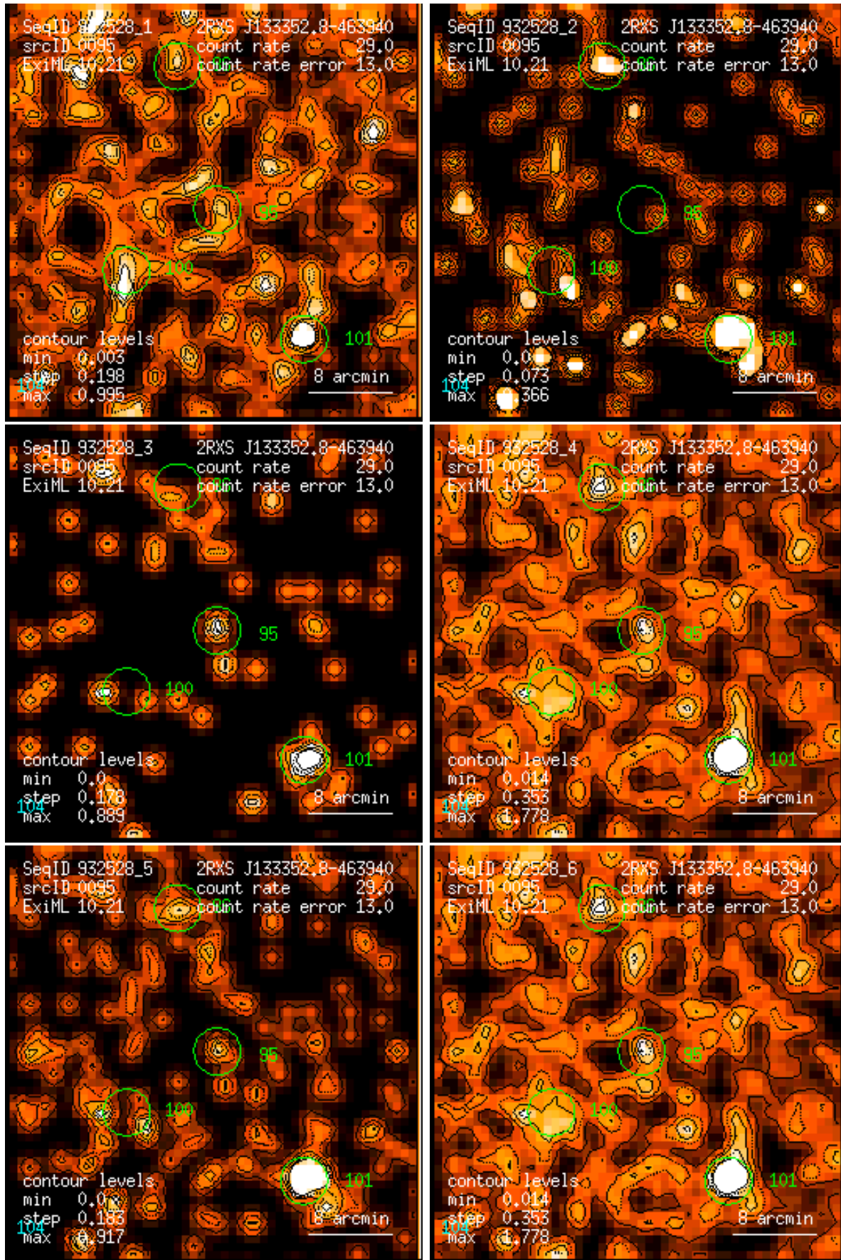
Figure 95: RASS 932528: detection 0095: band rate images, Gaussian filter: (1) PSPC channels 11 – 41, (2) 52 – 90, (3) 91 – 201, (4) 11 – 235, (5) 52 – 201, (6) 11 – 201. Broad band rates in counts/ks. Band rate contour levels in counts/ks/arcmin 2 .
