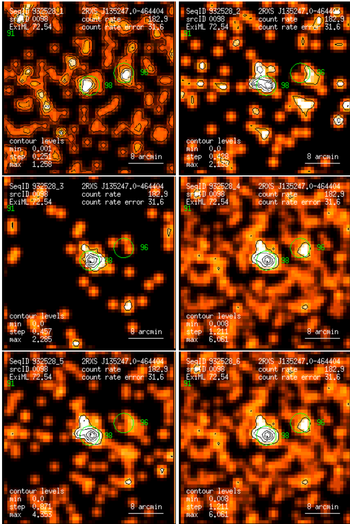
Figure 98: RASS 932528: detection 0098: band rate images, Gaussian filter: (1) PSPC channels 11 – 41, (2) 52 – 90, (3) 91 – 201, (4) 11 – 235, (5) 52 – 201, (6) 11 – 201. Broad band rates in counts/ks. Band rate contour levels in counts/ks/arcmin 2 .
