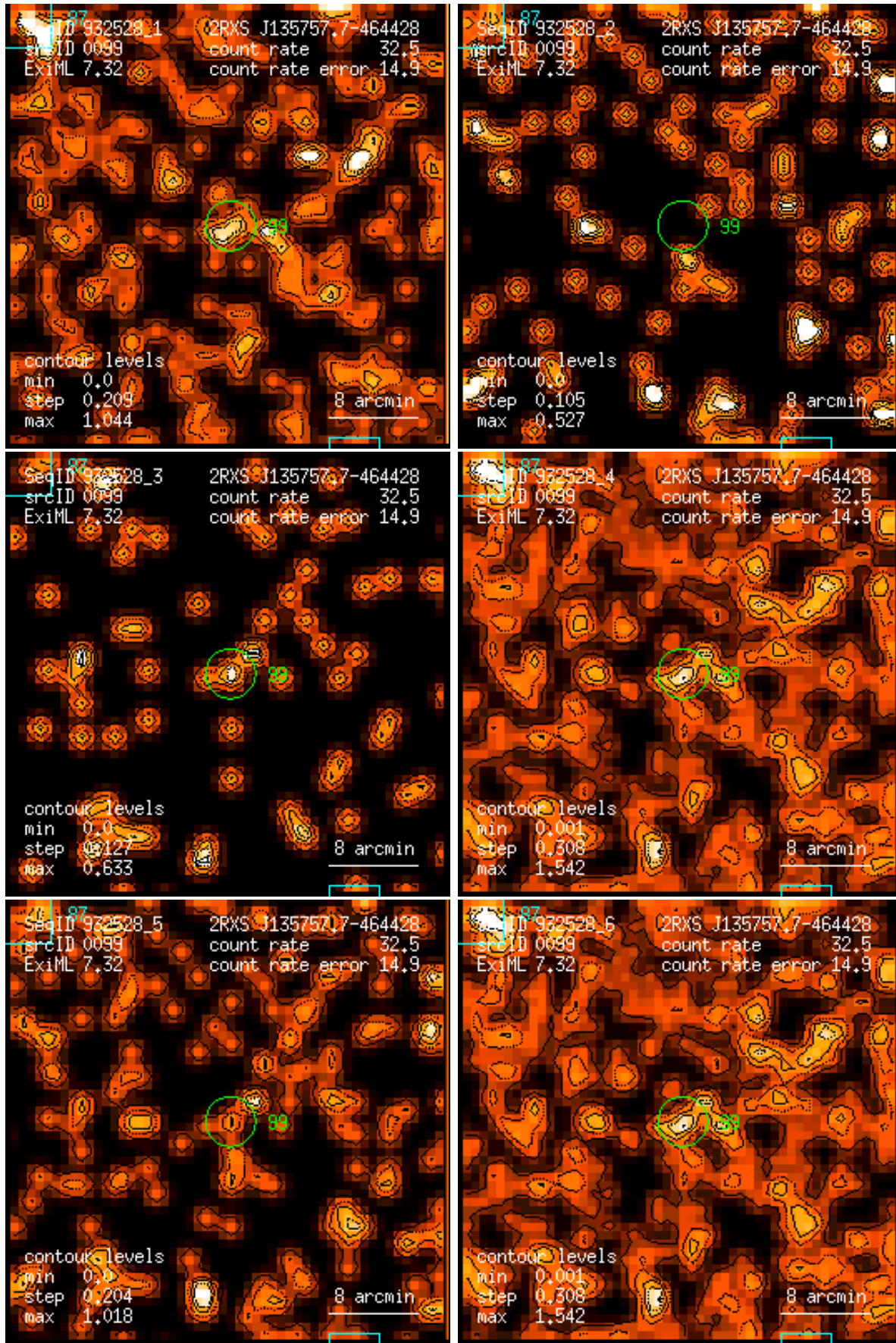
Figure 99: RASS 932528: detection 0099: band rate images, Gaussian filter: (1) PSPC channels 11 – 41, (2) 52 – 90, (3) 91 – 201, (4) 11 – 235, (5) 52 – 201, (6) 11 – 201. Broad band rates in counts/ks. Band rate contour levels in counts/ks/arcmin 2 .
