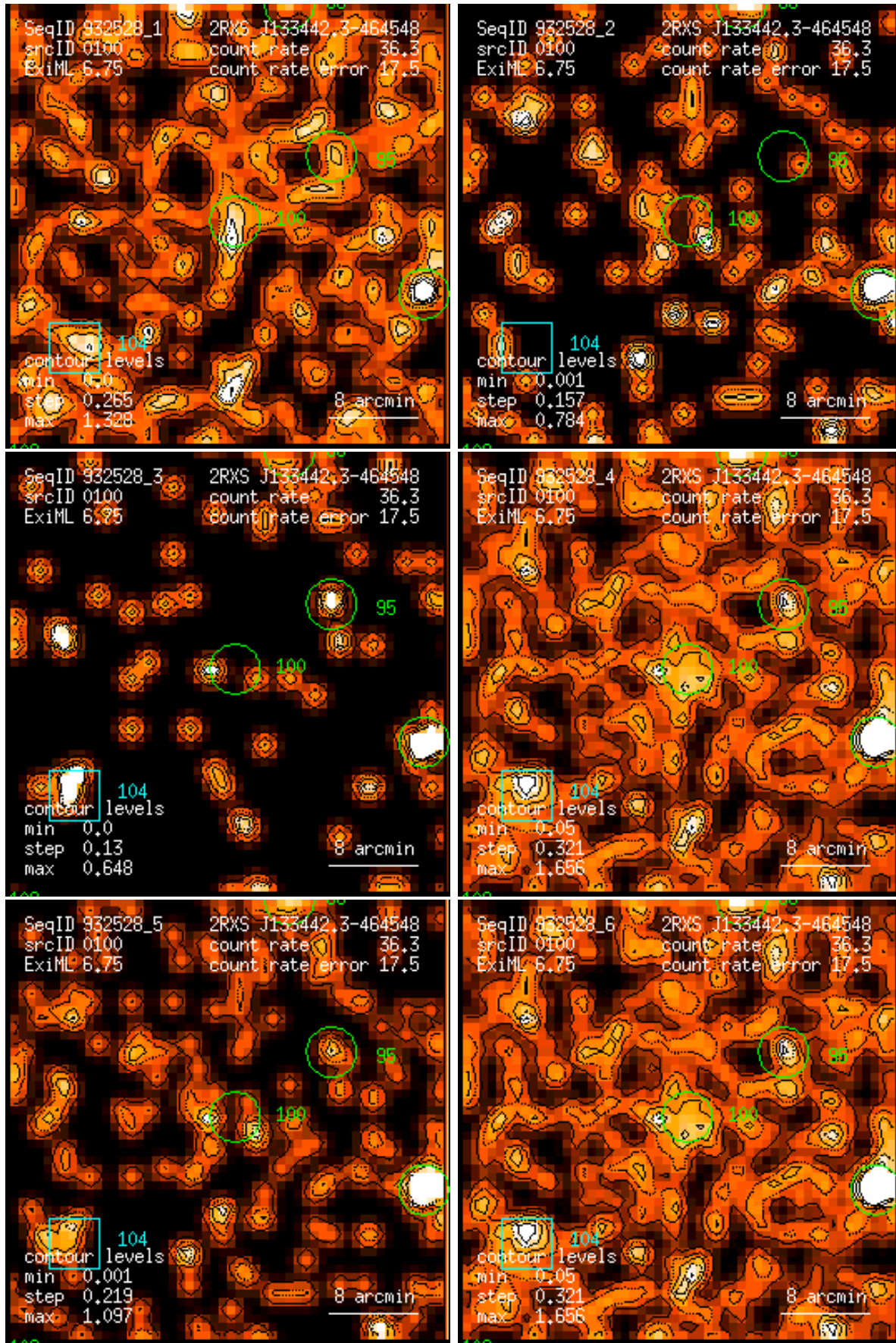
Figure 100: RASS 932528: detection 0100: band rate images, Gaussian filter: (1) PSPC channels 11 – 41, (2) 52 – 90, (3) 91 – 201, (4) 11 – 235, (5) 52 – 201, (6) 11 – 201. Broad band rates in counts/ks. Band rate contour levels in counts/ks/arcmin 2 .
