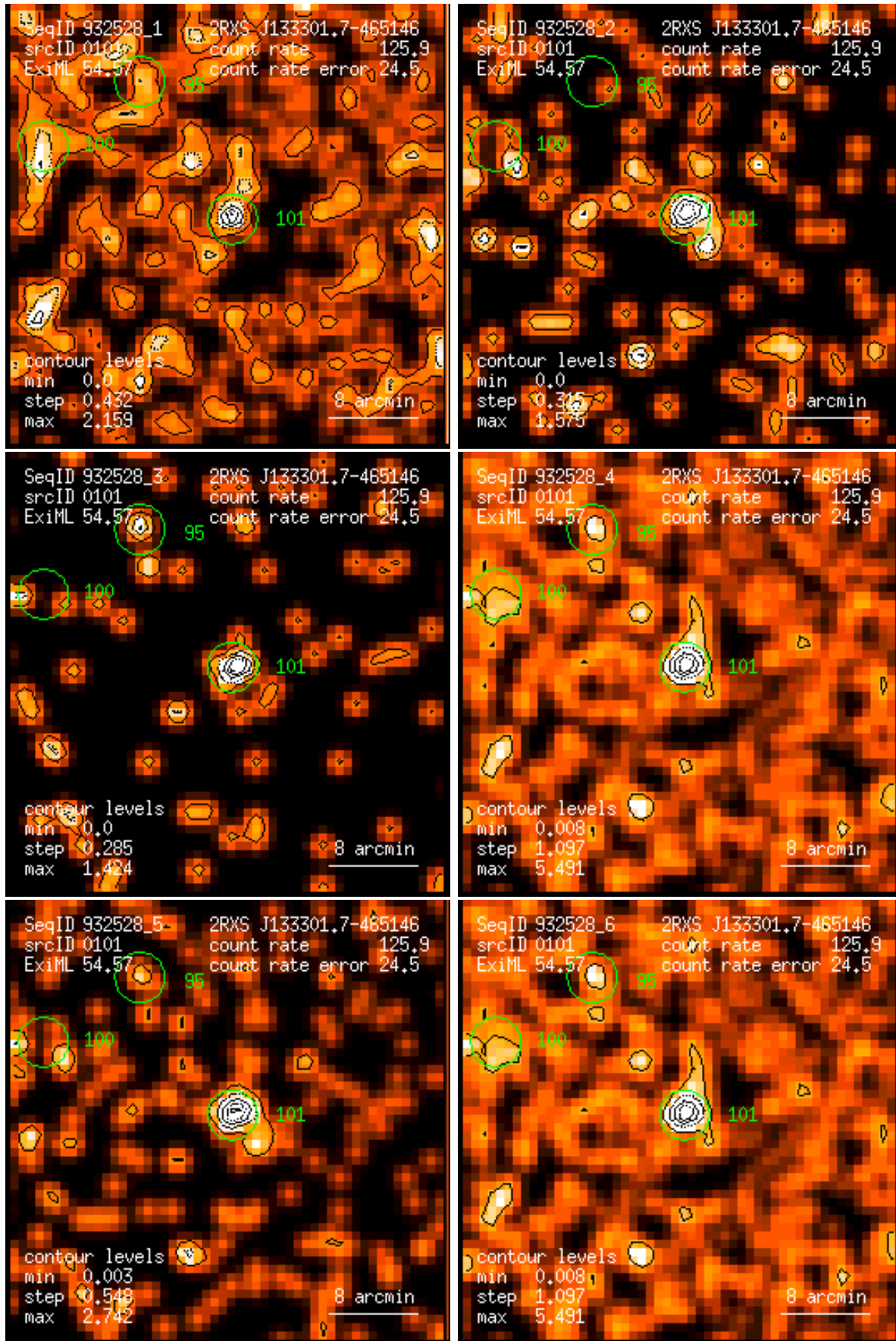
Figure 101: RASS 932528: detection 0101: band rate images, Gaussian filter: (1) PSPC channels 11 – 41, (2) 52 – 90, (3) 91 – 201, (4) 11 – 235, (5) 52 – 201, (6) 11 – 201. Broad band rates in counts/ks. Band rate contour levels in counts/ks/arcmin 2 .
