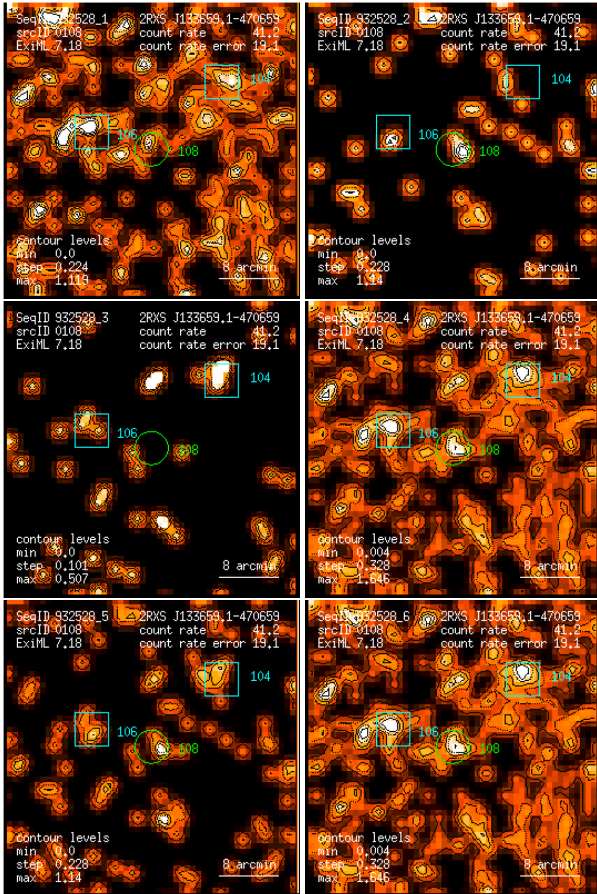
Figure 108: RASS 932528: detection 0108: band rate images, Gaussian filter: (1) PSPC channels 11 – 41, (2) 52 – 90, (3) 91 – 201, (4) 11 – 235, (5) 52 – 201, (6) 11 – 201. Broad band rates in counts/ks. Band rate contour levels in counts/ks/arcmin 2 .
