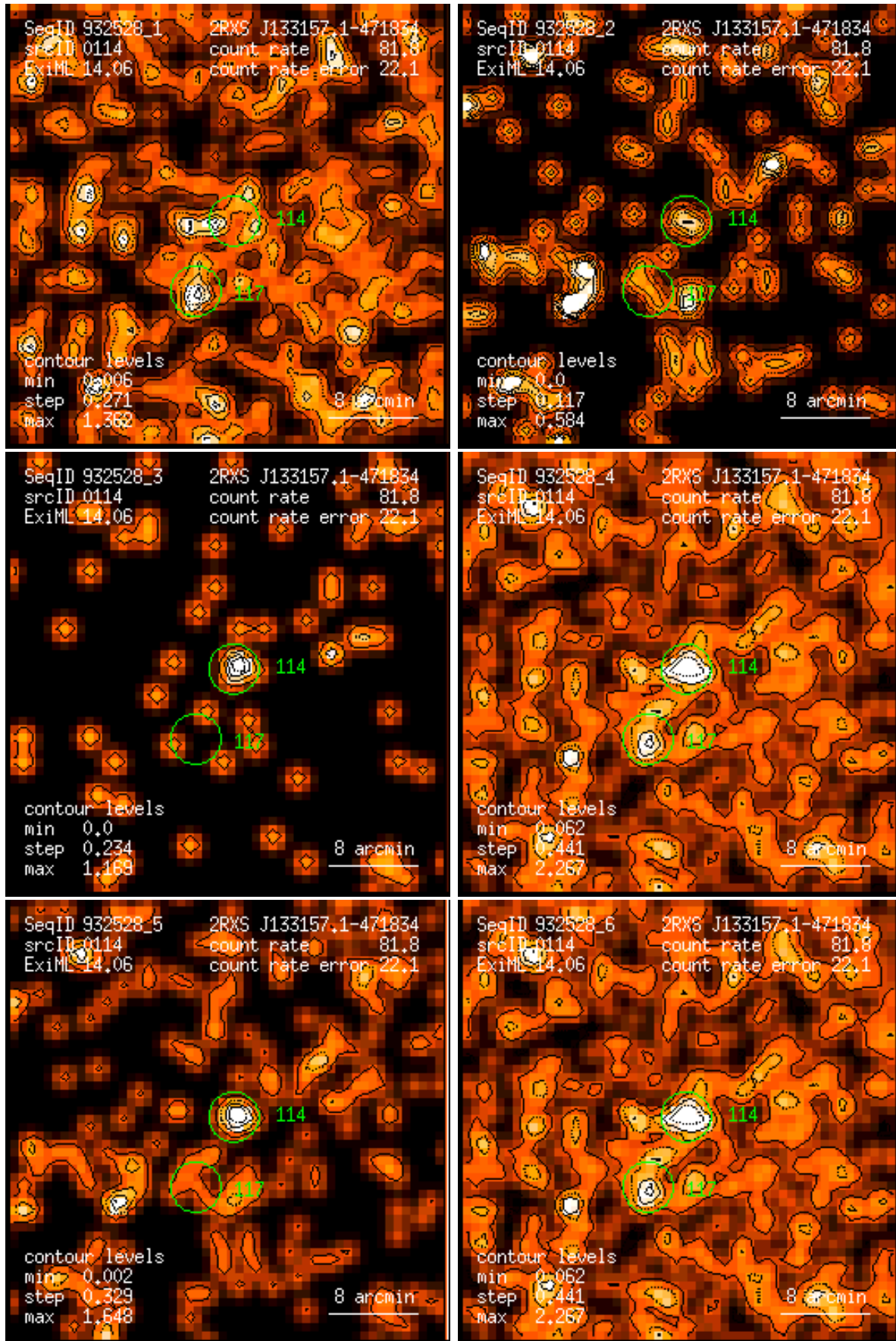
Figure 114: RASS 932528: detection 0114: band rate images, Gaussian filter: (1) PSPC channels 11 – 41, (2) 52 – 90, (3) 91 – 201, (4) 11 – 235, (5) 52 – 201, (6) 11 – 201. Broad band rates in counts/ks. Band rate contour levels in counts/ks/arcmin 2 .
