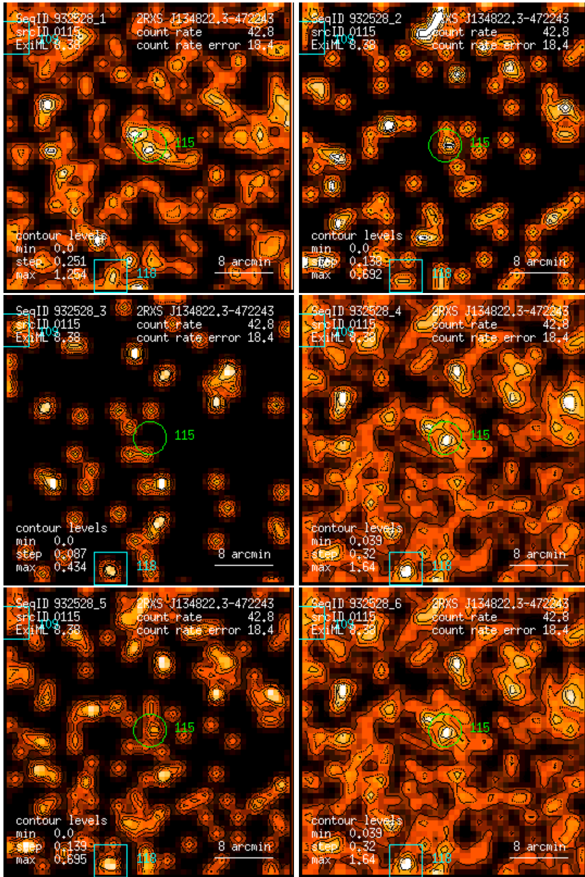
Figure 115: RASS 932528: detection 0115: band rate images, Gaussian filter: (1) PSPC channels 11 – 41, (2) 52 – 90, (3) 91 – 201, (4) 11 – 235, (5) 52 – 201, (6) 11 – 201. Broad band rates in counts/ks. Band rate contour levels in counts/ks/arcmin 2 .
