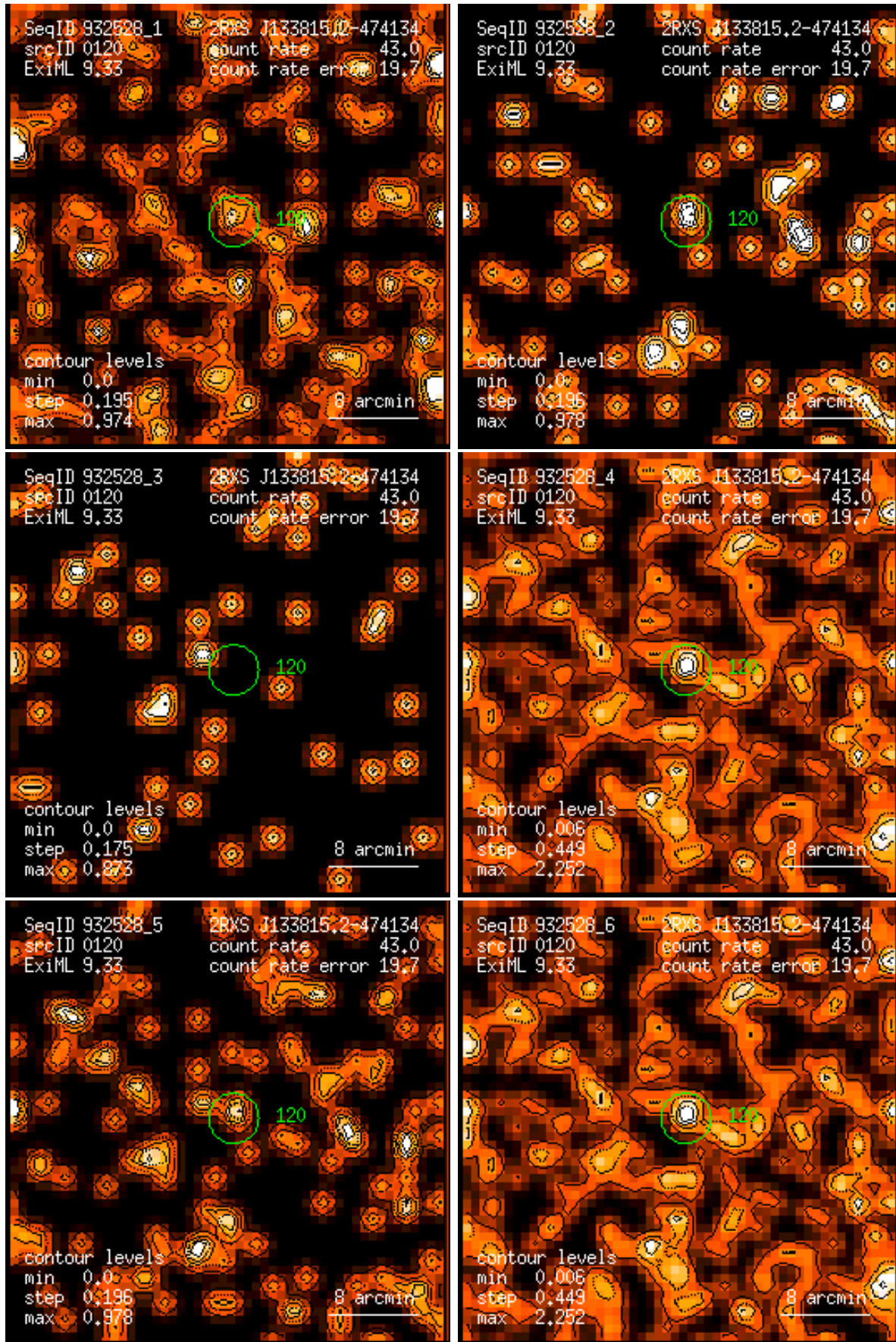
Figure 120: RASS 932528: detection 0120: band rate images, Gaussian filter: (1) PSPC channels 11 – 41, (2) 52 – 90, (3) 91 – 201, (4) 11 – 235, (5) 52 – 201, (6) 11 – 201. Broad band rates in counts/ks. Band rate contour levels in counts/ks/arcmin 2 .
