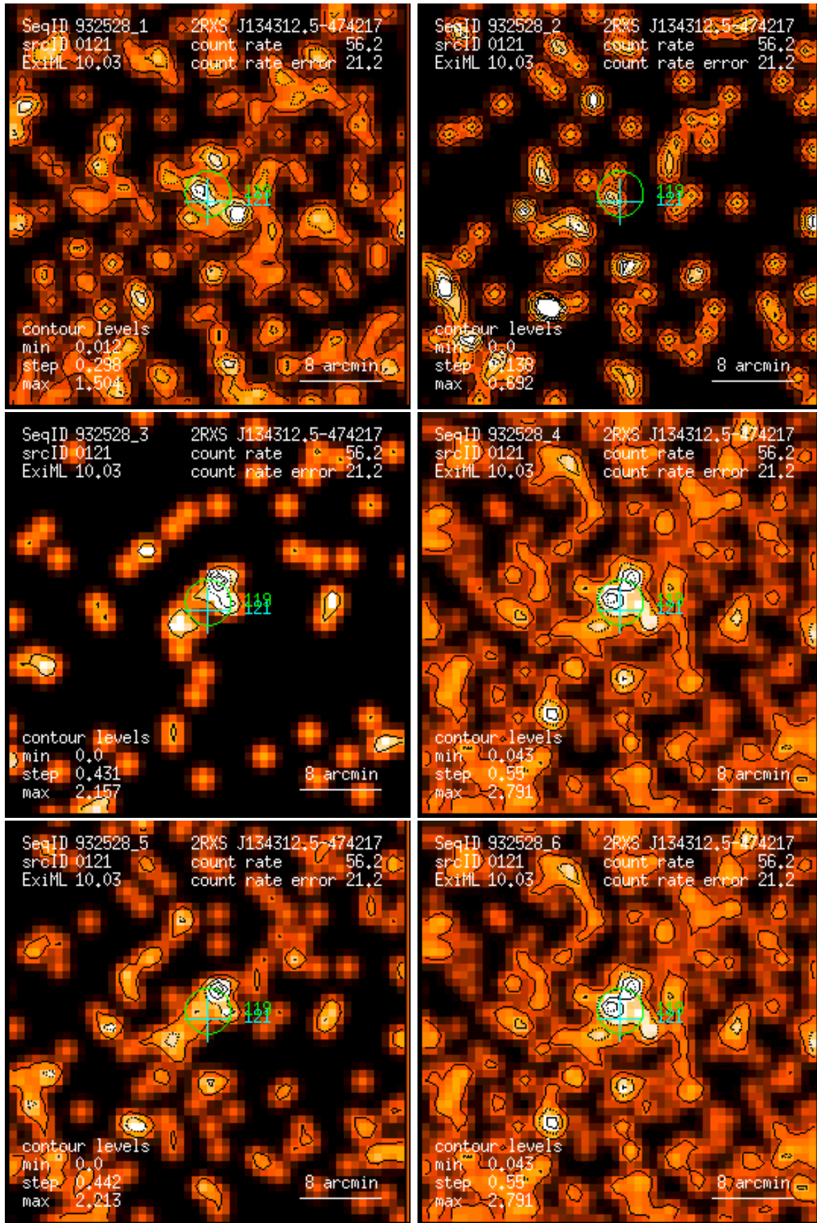
Figure 121: RASS 932528: detection 0121: band rate images, Gaussian filter: (1) PSPC channels 11 – 41, (2) 52 – 90, (3) 91 – 201, (4) 11 – 235, (5) 52 – 201, (6) 11 – 201. Broad band rates in counts/ks. Band rate contour levels in counts/ks/arcmin 2 .
