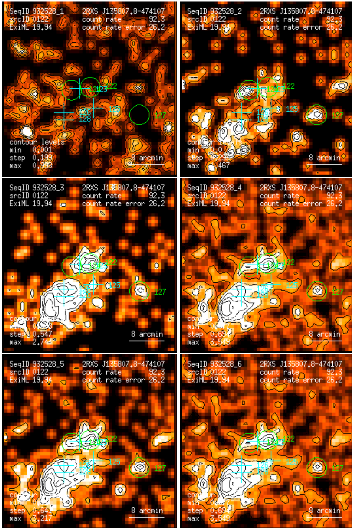
Figure 122: RASS 932528: detection 0122: band rate images, Gaussian filter: (1) PSPC channels 11 – 41, (2) 52 – 90, (3) 91 – 201, (4) 11 – 235, (5) 52 – 201, (6) 11 – 201. Broad band rates in counts/ks. Band rate contour levels in counts/ks/arcmin 2 .
