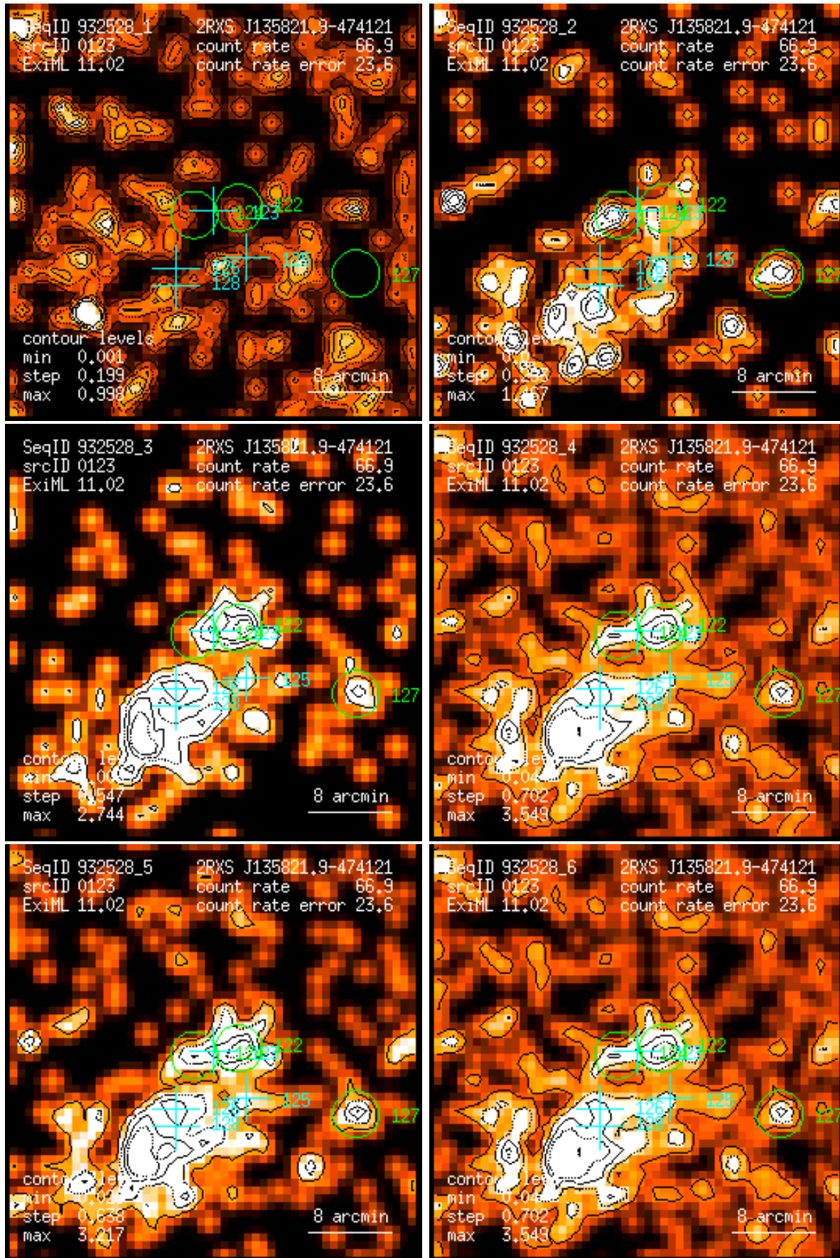
Figure 123: RASS 932528: detection 0123: band rate images, Gaussian filter: (1) PSPC channels 11 – 41, (2) 52 – 90, (3) 91 – 201, (4) 11 – 235, (5) 52 – 201, (6) 11 – 201. Broad band rates in counts/ks. Band rate contour levels in counts/ks/arcmin 2 .
