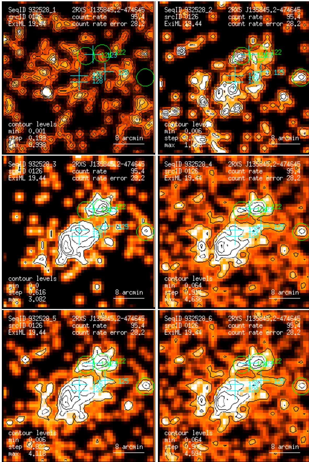
Figure 126: RASS 932528: detection 0126: band rate images, Gaussian filter: (1) PSPC channels 11 – 41, (2) 52 – 90, (3) 91 – 201, (4) 11 – 235, (5) 52 – 201, (6) 11 – 201. Broad band rates in counts/ks. Band rate contour levels in counts/ks/arcmin 2 .
