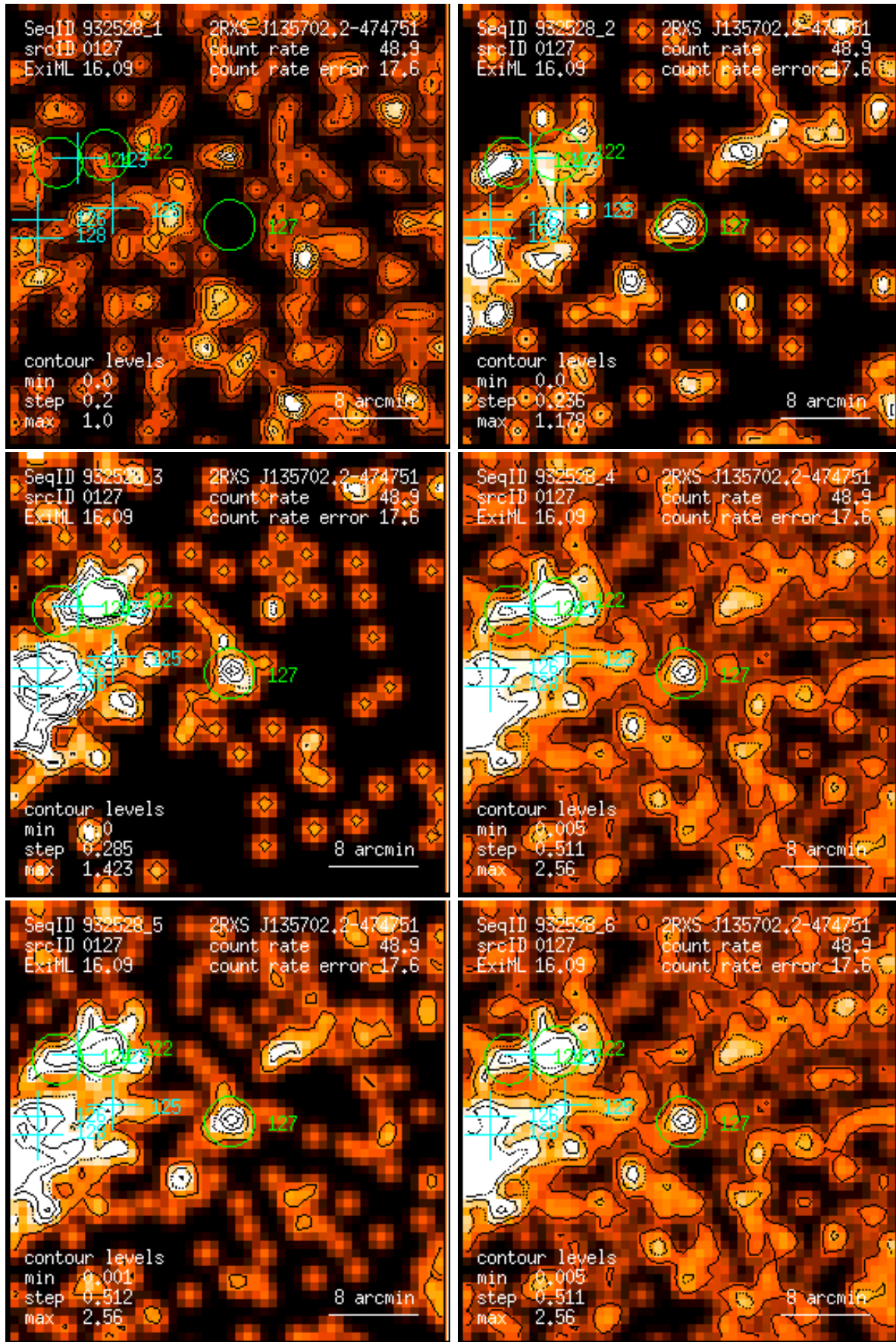
Figure 127: RASS 932528: detection 0127: band rate images, Gaussian filter: (1) PSPC channels 11 – 41, (2) 52 – 90, (3) 91 – 201, (4) 11 – 235, (5) 52 – 201, (6) 11 – 201. Broad band rates in counts/ks. Band rate contour levels in counts/ks/arcmin 2 .
