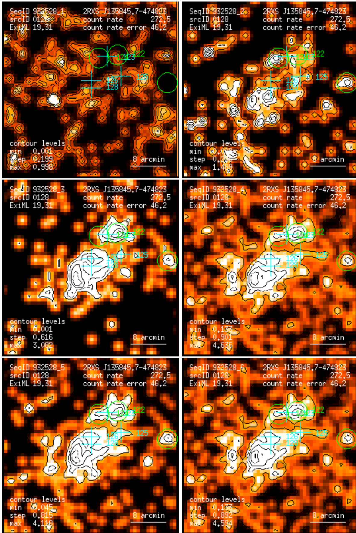
Figure 128: RASS 932528: detection 0128: band rate images, Gaussian filter: (1) PSPC channels 11 – 41, (2) 52 – 90, (3) 91 – 201, (4) 11 – 235, (5) 52 – 201, (6) 11 – 201. Broad band rates in counts/ks. Band rate contour levels in counts/ks/arcmin 2 .
