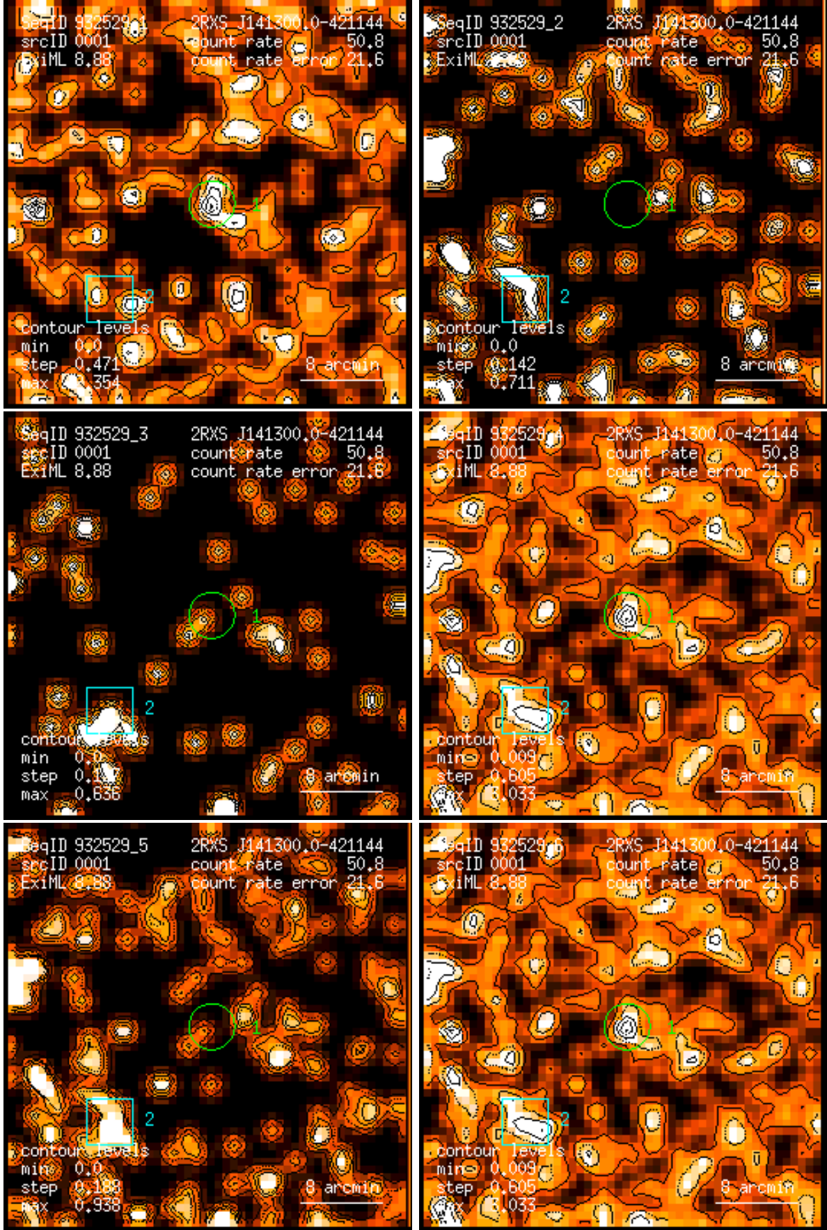
Figure 1: RASS 932529: detection 0001: band rate images, Gaussian filter: (1) PSPC channels 11 – 41, (2) 52 – 90, (3) 91 – 201, (4) 11 – 235, (5) 52 – 201, (6) 11 – 201. Broad band rates in counts/ks. Band rate contour levels in counts/ks/arcmin 2 .
