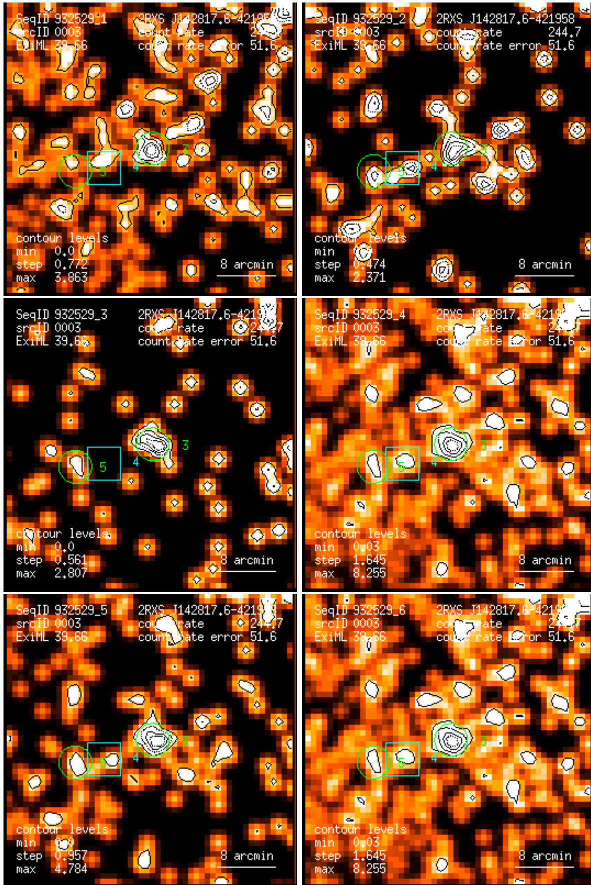
Figure 3: RASS 932529: detection 0003: band rate images, Gaussian filter: (1) PSPC channels 11 – 41, (2) 52 – 90, (3) 91 – 201, (4) 11 – 235, (5) 52 – 201, (6) 11 – 201. Broad band rates in counts/ks. Band rate contour levels in counts/ks/arcmin 2 .
