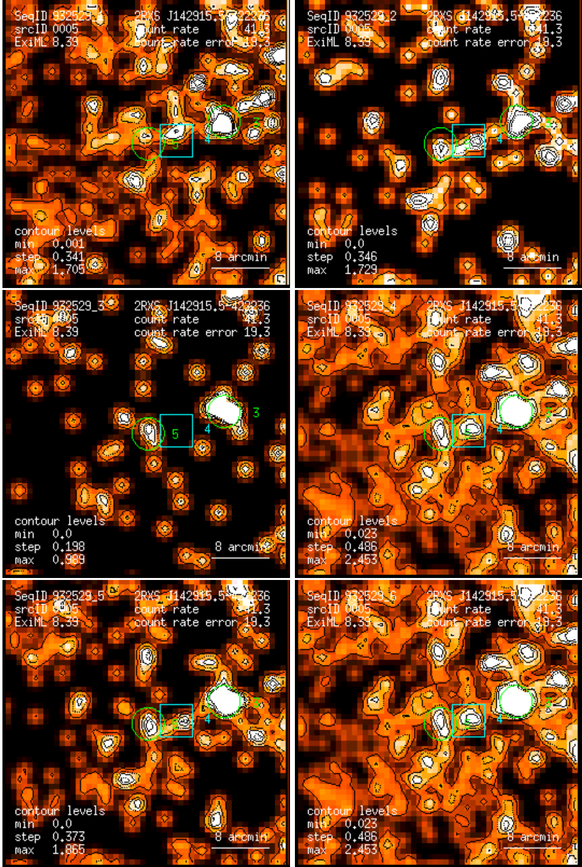
Figure 5: RASS 932529: detection 0005: band rate images, Gaussian filter: (1) PSPC channels 11 – 41, (2) 52 – 90, (3) 91 – 201, (4) 11 – 235, (5) 52 – 201, (6) 11 – 201. Broad band rates in counts/ks. Band rate contour levels in counts/ks/arcmin 2 .
