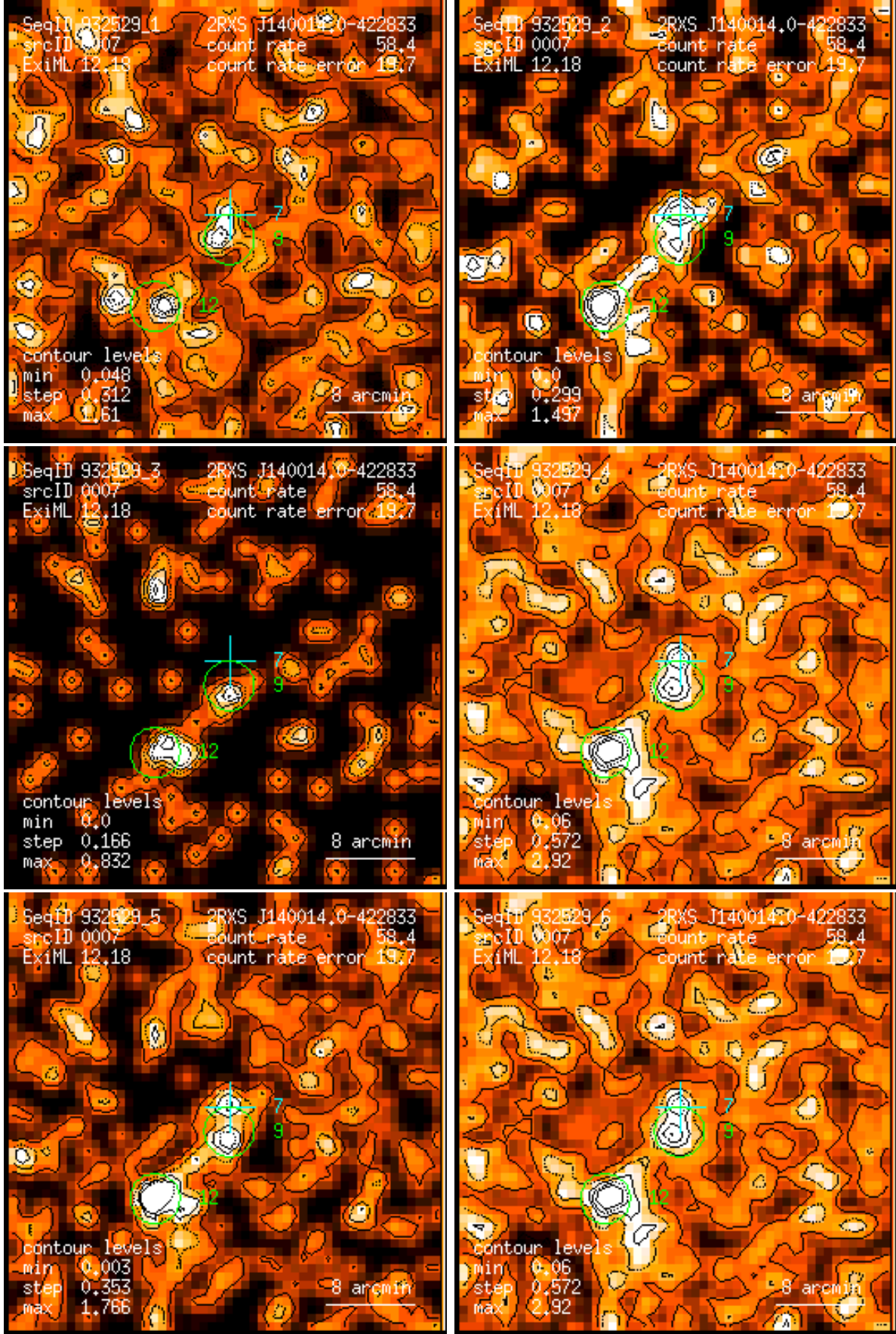
Figure 7: RASS 932529: detection 0007: band rate images, Gaussian filter: (1) PSPC channels 11 – 41, (2) 52 – 90, (3) 91 – 201, (4) 11 – 235, (5) 52 – 201, (6) 11 – 201. Broad band rates in counts/ks. Band rate contour levels in counts/ks/arcmin 2 .
