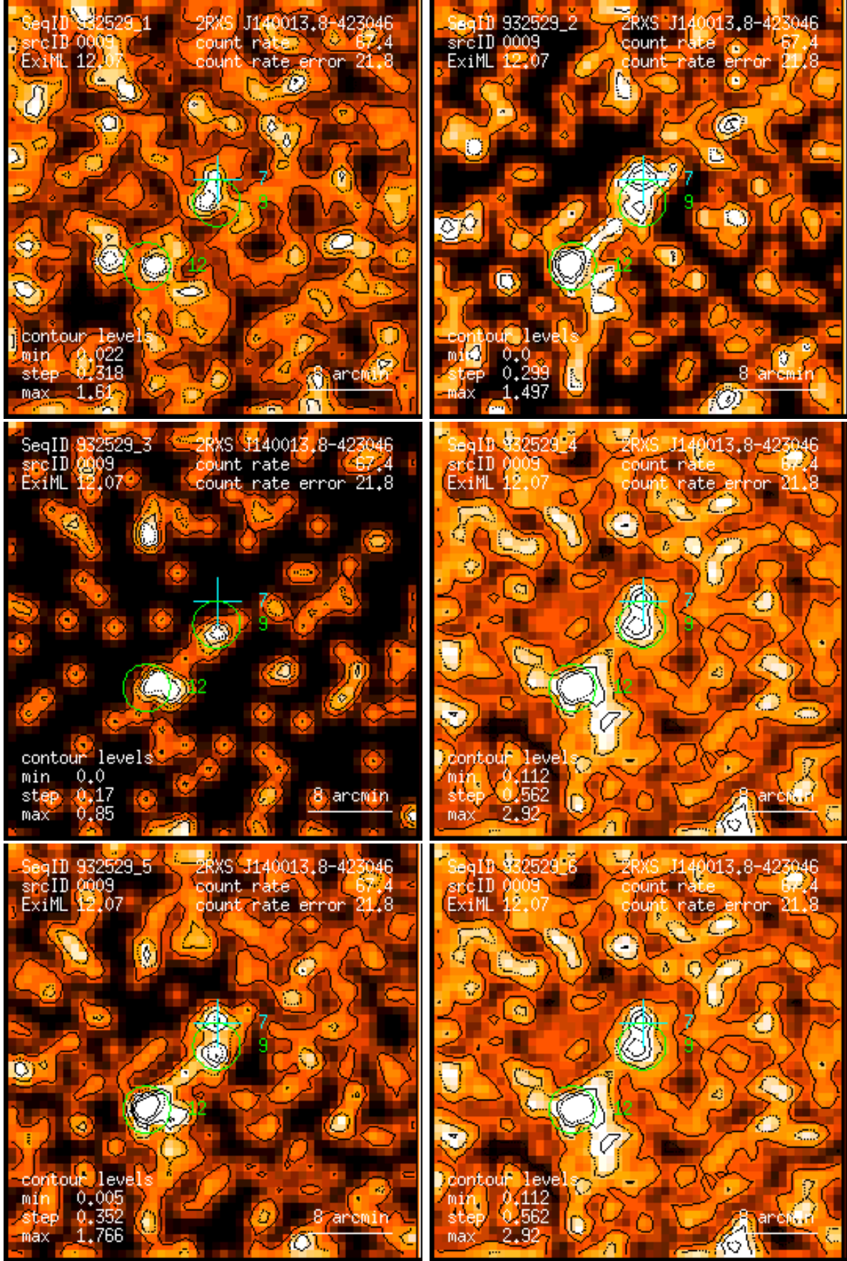
Figure 9: RASS 932529: detection 0009: band rate images, Gaussian filter: (1) PSPC channels 11 – 41, (2) 52 – 90, (3) 91 – 201, (4) 11 – 235, (5) 52 – 201, (6) 11 – 201. Broad band rates in counts/ks. Band rate contour levels in counts/ks/arcmin 2 .
