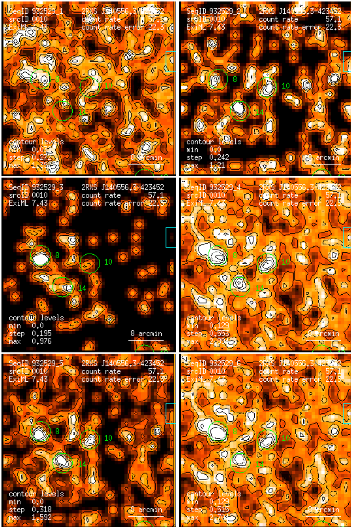
Figure 10: RASS 932529: detection 0010: band rate images, Gaussian filter: (1) PSPC channels 11 – 41, (2) 52 – 90, (3) 91 – 201, (4) 11 – 235, (5) 52 – 201, (6) 11 – 201. Broad band rates in counts/ks. Band rate contour levels in counts/ks/arcmin 2 .
