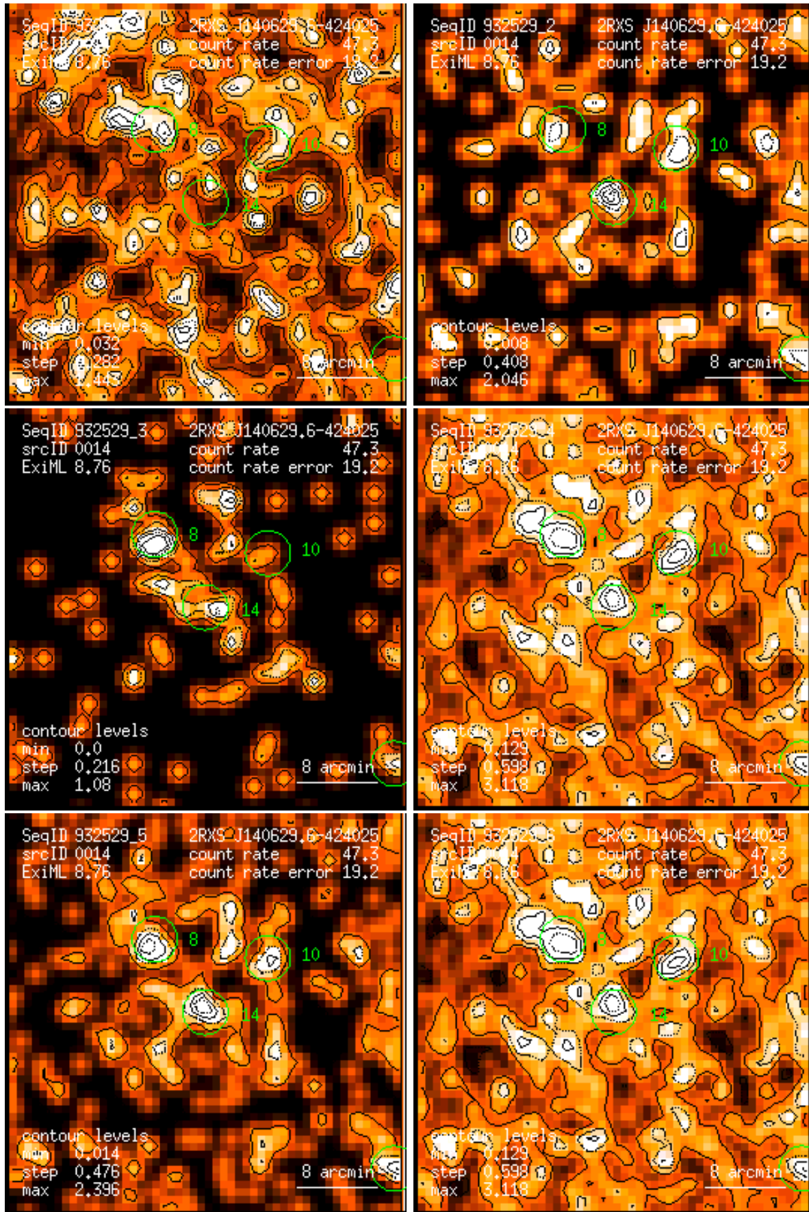
Figure 14: RASS 932529: detection 0014: band rate images, Gaussian filter: (1) PSPC channels 11 – 41, (2) 52 – 90, (3) 91 – 201, (4) 11 – 235, (5) 52 – 201, (6) 11 – 201. Broad band rates in counts/ks. Band rate contour levels in counts/ks/arcmin 2 .
