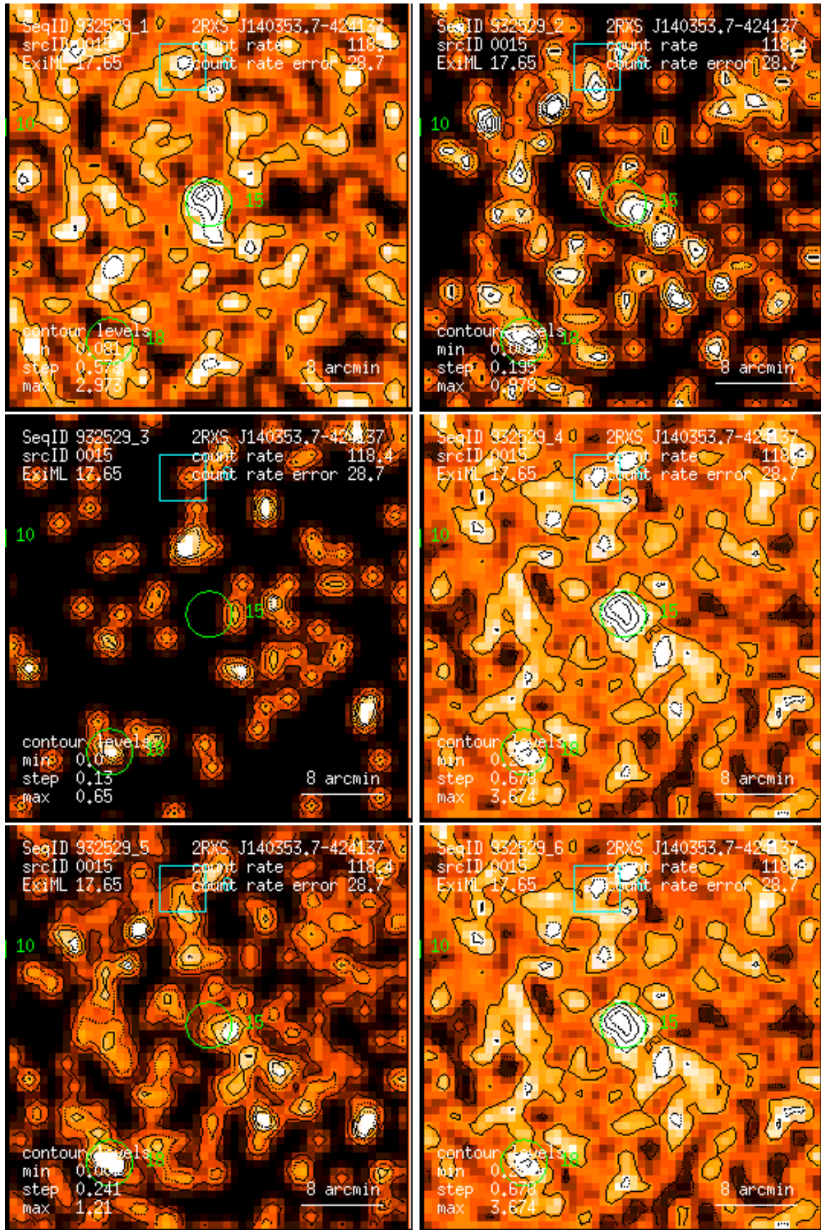
Figure 15: RASS 932529: detection 0015: band rate images, Gaussian filter: (1) PSPC channels 11 – 41, (2) 52 – 90, (3) 91 – 201, (4) 11 – 235, (5) 52 – 201, (6) 11 – 201. Broad band rates in counts/ks. Band rate contour levels in counts/ks/arcmin 2 .
