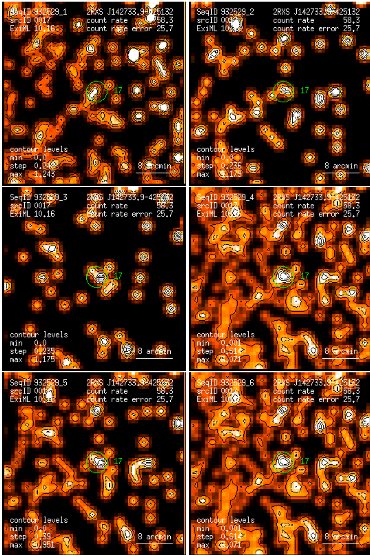
Figure 17: RASS 932529: detection 0017: band rate images, Gaussian filter: (1) PSPC channels 11 – 41, (2) 52 – 90, (3) 91 – 201, (4) 11 – 235, (5) 52 – 201, (6) 11 – 201. Broad band rates in counts/ks. Band rate contour levels in counts/ks/arcmin 2 .
