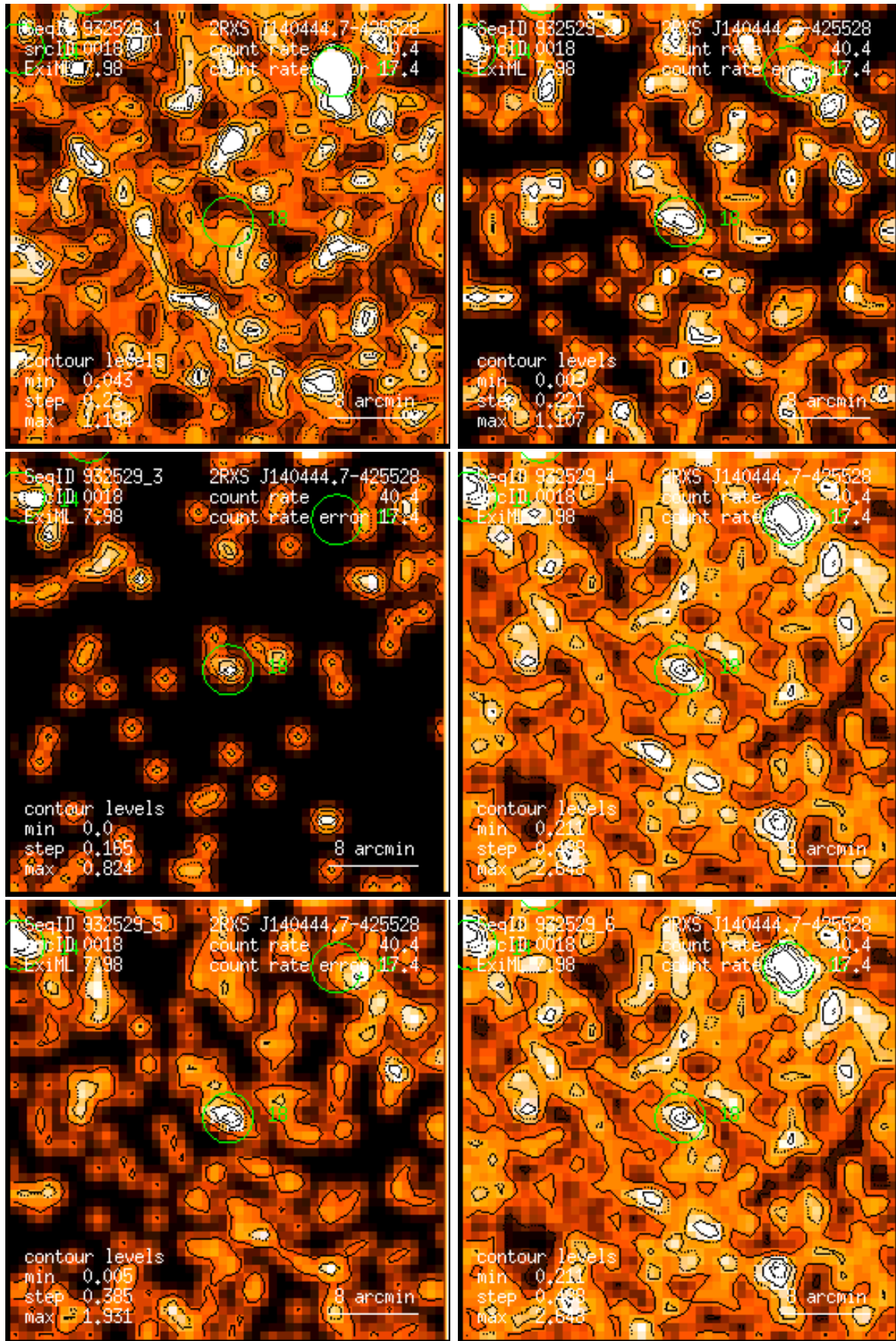
Figure 18: RASS 932529: detection 0018: band rate images, Gaussian filter: (1) PSPC channels 11 – 41, (2) 52 – 90, (3) 91 – 201, (4) 11 – 235, (5) 52 – 201, (6) 11 – 201. Broad band rates in counts/ks. Band rate contour levels in counts/ks/arcmin 2 .
