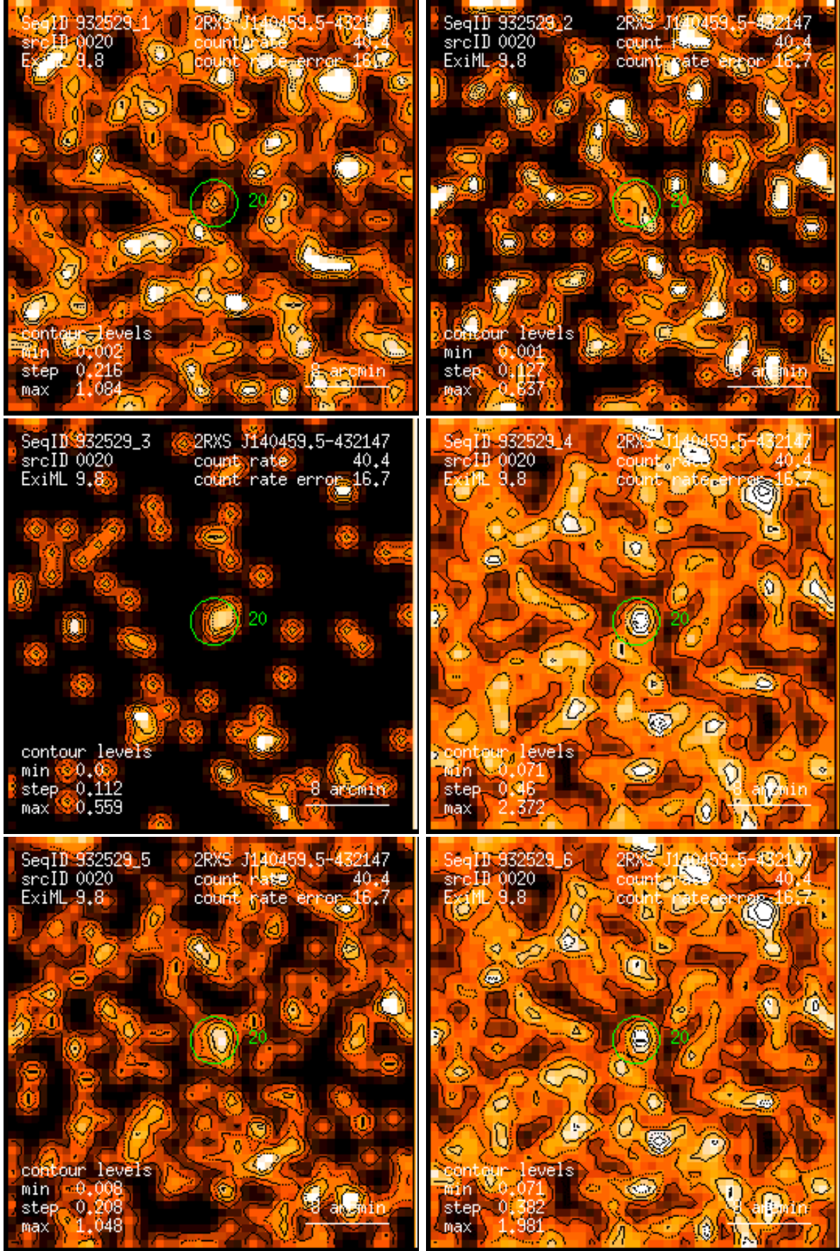
Figure 20: RASS 932529: detection 0020: band rate images, Gaussian filter: (1) PSPC channels 11 – 41, (2) 52 – 90, (3) 91 – 201, (4) 11 – 235, (5) 52 – 201, (6) 11 – 201. Broad band rates in counts/ks. Band rate contour levels in counts/ks/arcmin 2 .
