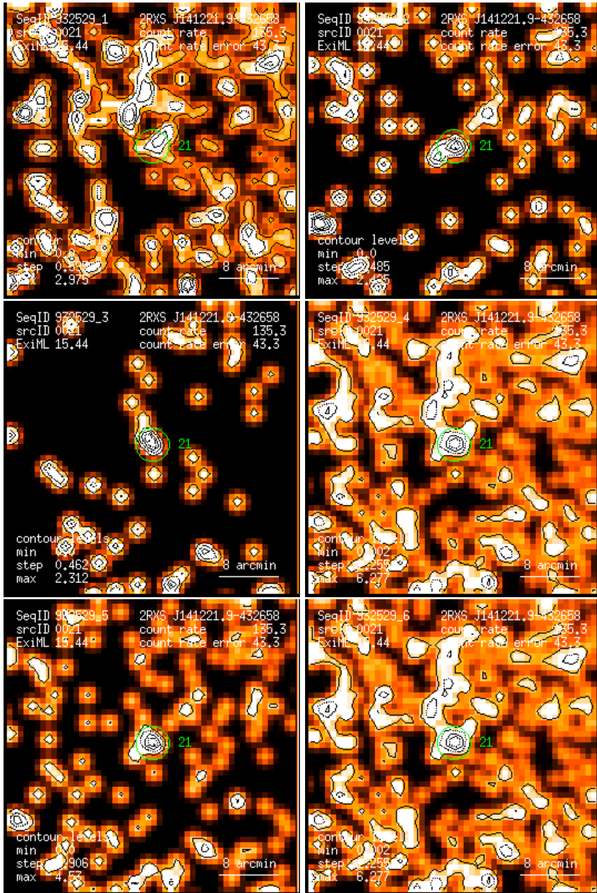
Figure 21: RASS 932529: detection 0021: band rate images, Gaussian filter: (1) PSPC channels 11 – 41, (2) 52 – 90, (3) 91 – 201, (4) 11 – 235, (5) 52 – 201, (6) 11 – 201. Broad band rates in counts/ks. Band rate contour levels in counts/ks/arcmin 2 .
