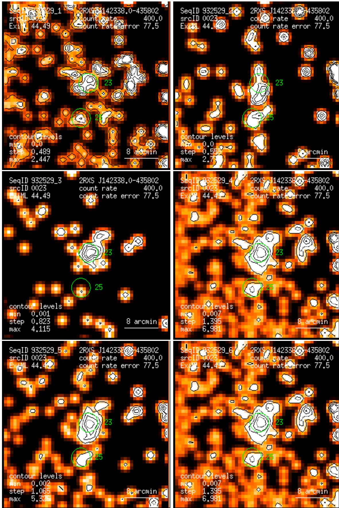
Figure 23: RASS 932529: detection 0023: band rate images, Gaussian filter: (1) PSPC channels 11 – 41, (2) 52 – 90, (3) 91 – 201, (4) 11 – 235, (5) 52 – 201, (6) 11 – 201. Broad band rates in counts/ks. Band rate contour levels in counts/ks/arcmin 2 .
