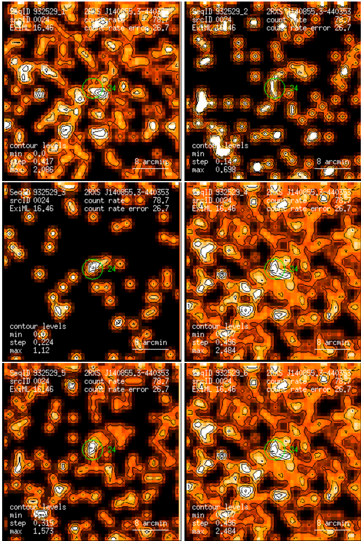
Figure 24: RASS 932529: detection 0024: band rate images, Gaussian filter: (1) PSPC channels 11 – 41, (2) 52 – 90, (3) 91 – 201, (4) 11 – 235, (5) 52 – 201, (6) 11 – 201. Broad band rates in counts/ks. Band rate contour levels in counts/ks/arcmin 2 .
