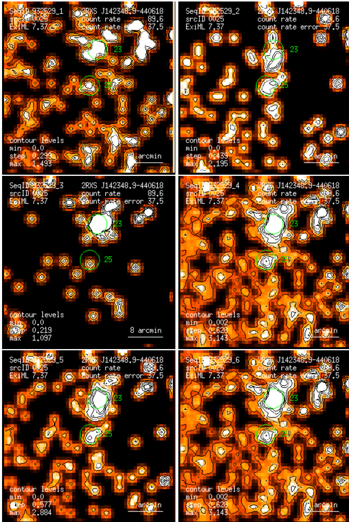
Figure 25: RASS 932529: detection 0025: band rate images, Gaussian filter: (1) PSPC channels 11 – 41, (2) 52 – 90, (3) 91 – 201, (4) 11 – 235, (5) 52 – 201, (6) 11 – 201. Broad band rates in counts/ks. Band rate contour levels in counts/ks/arcmin 2 .
