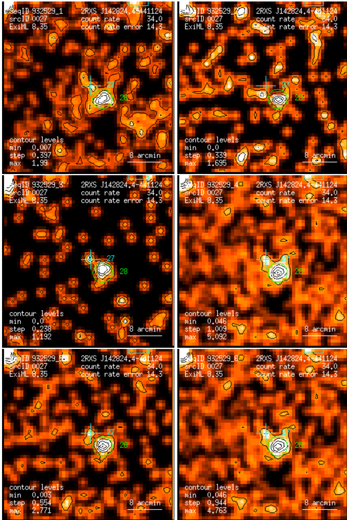
Figure 27: RASS 932529: detection 0027: band rate images, Gaussian filter: (1) PSPC channels 11 – 41, (2) 52 – 90, (3) 91 – 201, (4) 11 – 235, (5) 52 – 201, (6) 11 – 201. Broad band rates in counts/ks. Band rate contour levels in counts/ks/arcmin 2 .
