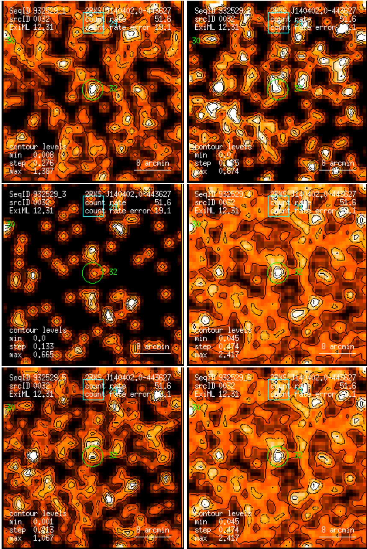
Figure 32: RASS 932529: detection 0032: band rate images, Gaussian filter: (1) PSPC channels 11 – 41, (2) 52 – 90, (3) 91 – 201, (4) 11 – 235, (5) 52 – 201, (6) 11 – 201. Broad band rates in counts/ks. Band rate contour levels in counts/ks/arcmin 2 .
