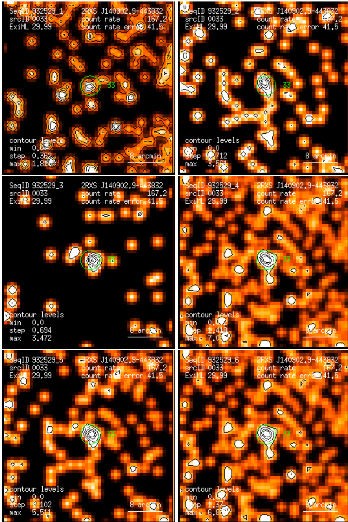
Figure 33: RASS 932529: detection 0033: band rate images, Gaussian filter: (1) PSPC channels 11 – 41, (2) 52 – 90, (3) 91 – 201, (4) 11 – 235, (5) 52 – 201, (6) 11 – 201. Broad band rates in counts/ks. Band rate contour levels in counts/ks/arcmin 2 .
