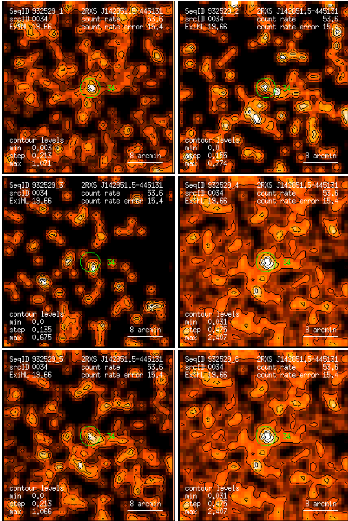
Figure 34: RASS 932529: detection 0034: band rate images, Gaussian filter: (1) PSPC channels 11 – 41, (2) 52 – 90, (3) 91 – 201, (4) 11 – 235, (5) 52 – 201, (6) 11 – 201. Broad band rates in counts/ks. Band rate contour levels in counts/ks/arcmin 2 .
