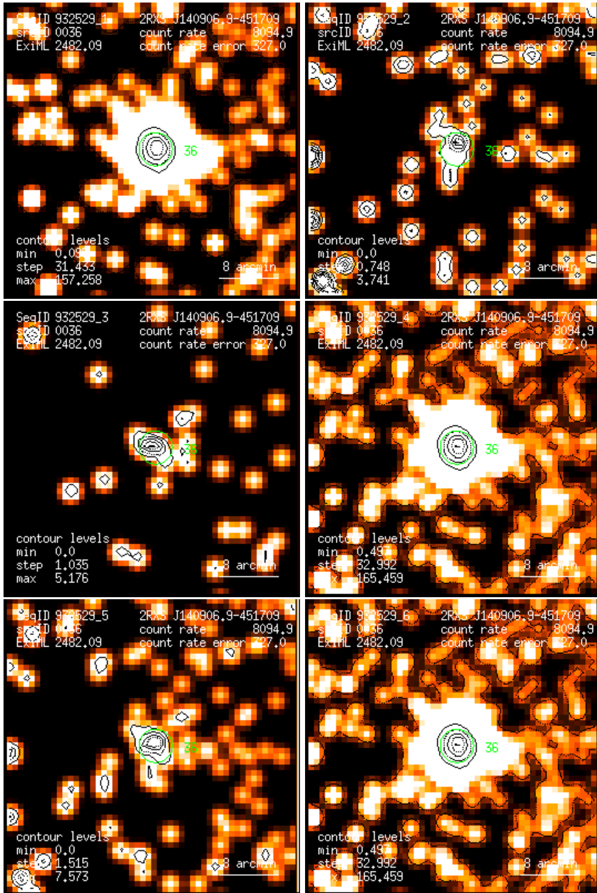
Figure 36: RASS 932529: detection 0036: band rate images, Gaussian filter: (1) PSPC channels 11 – 41, (2) 52 – 90, (3) 91 – 201, (4) 11 – 235, (5) 52 – 201, (6) 11 – 201. Broad band rates in counts/ks. Band rate contour levels in counts/ks/arcmin 2 .
