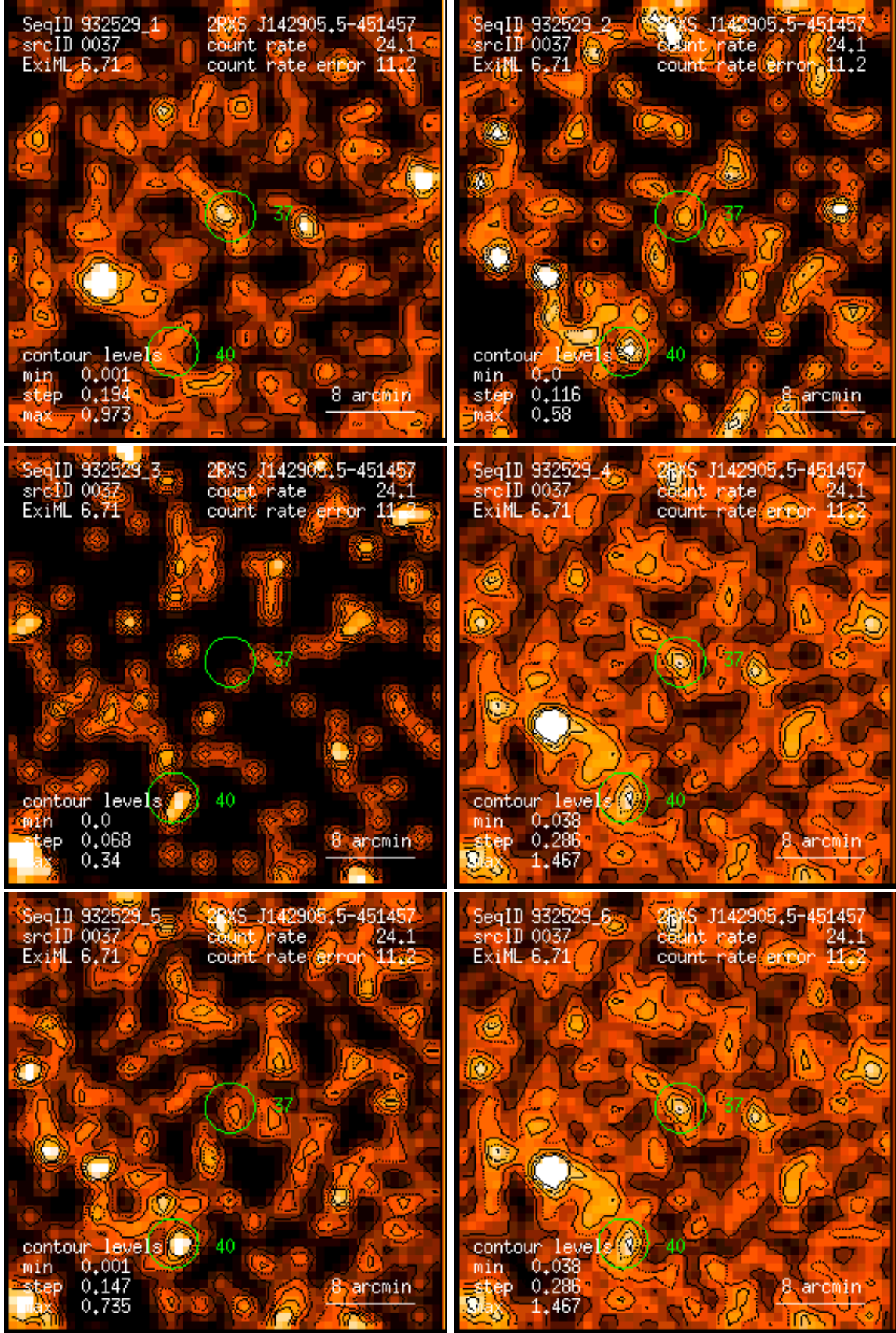
Figure 37: RASS 932529: detection 0037: band rate images, Gaussian filter: (1) PSPC channels 11 – 41, (2) 52 – 90, (3) 91 – 201, (4) 11 – 235, (5) 52 – 201, (6) 11 – 201. Broad band rates in counts/ks. Band rate contour levels in counts/ks/arcmin 2 .
