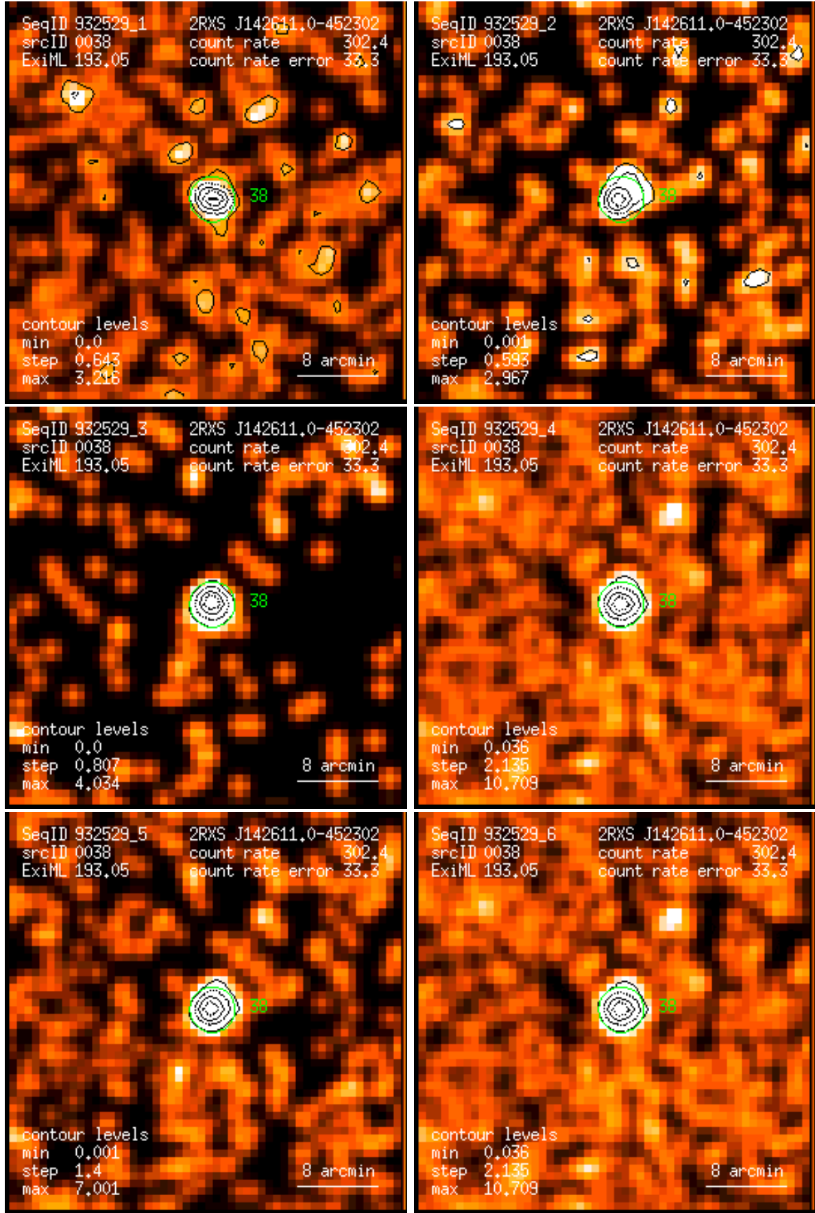
Figure 38: RASS 932529: detection 0038: band rate images, Gaussian filter: (1) PSPC channels 11 – 41, (2) 52 – 90, (3) 91 – 201, (4) 11 – 235, (5) 52 – 201, (6) 11 – 201. Broad band rates in counts/ks. Band rate contour levels in counts/ks/arcmin 2 .
